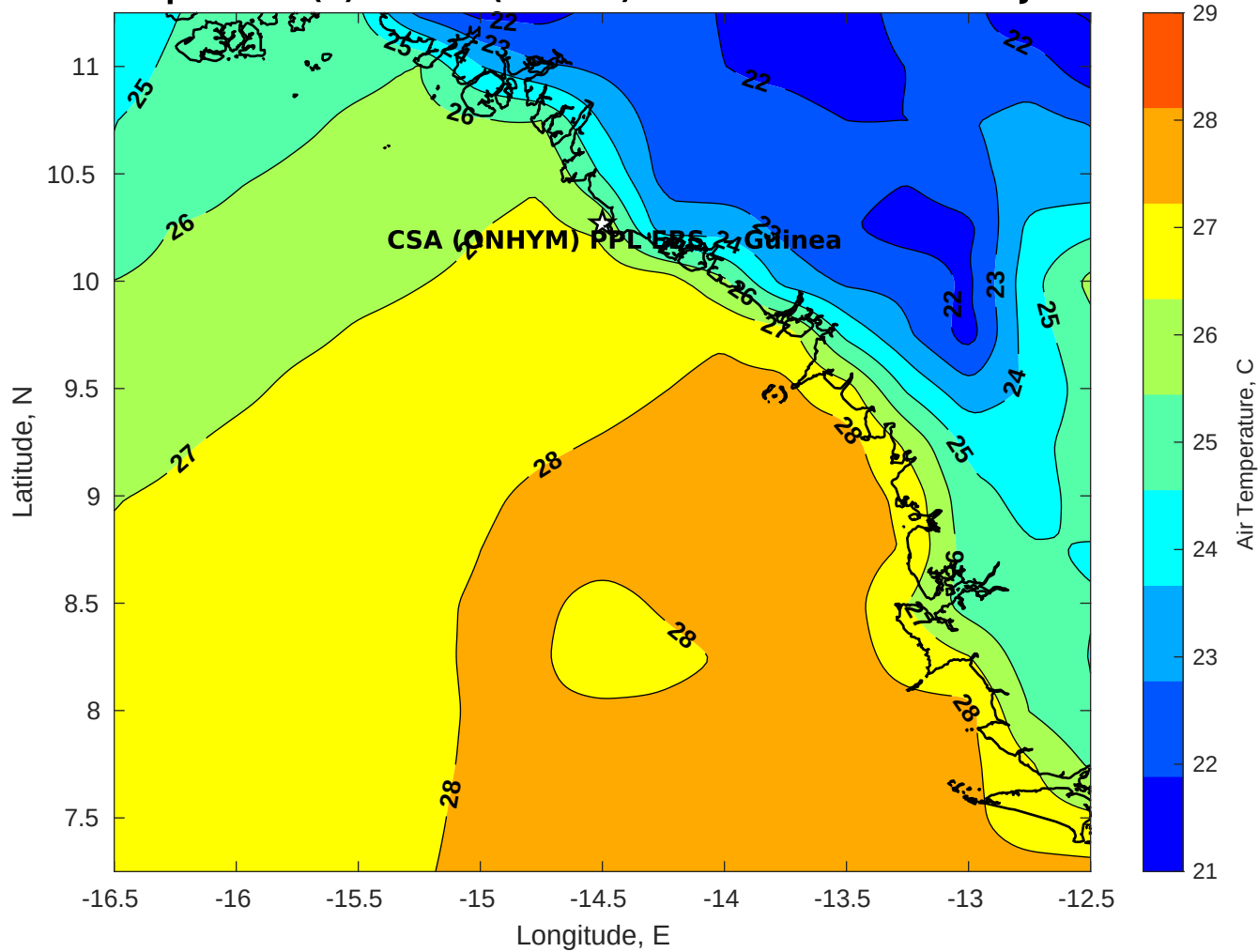
Air Temperature (C) for CSA (ONHYM) PPL EBS - Guinea at 22-Jan-2026
