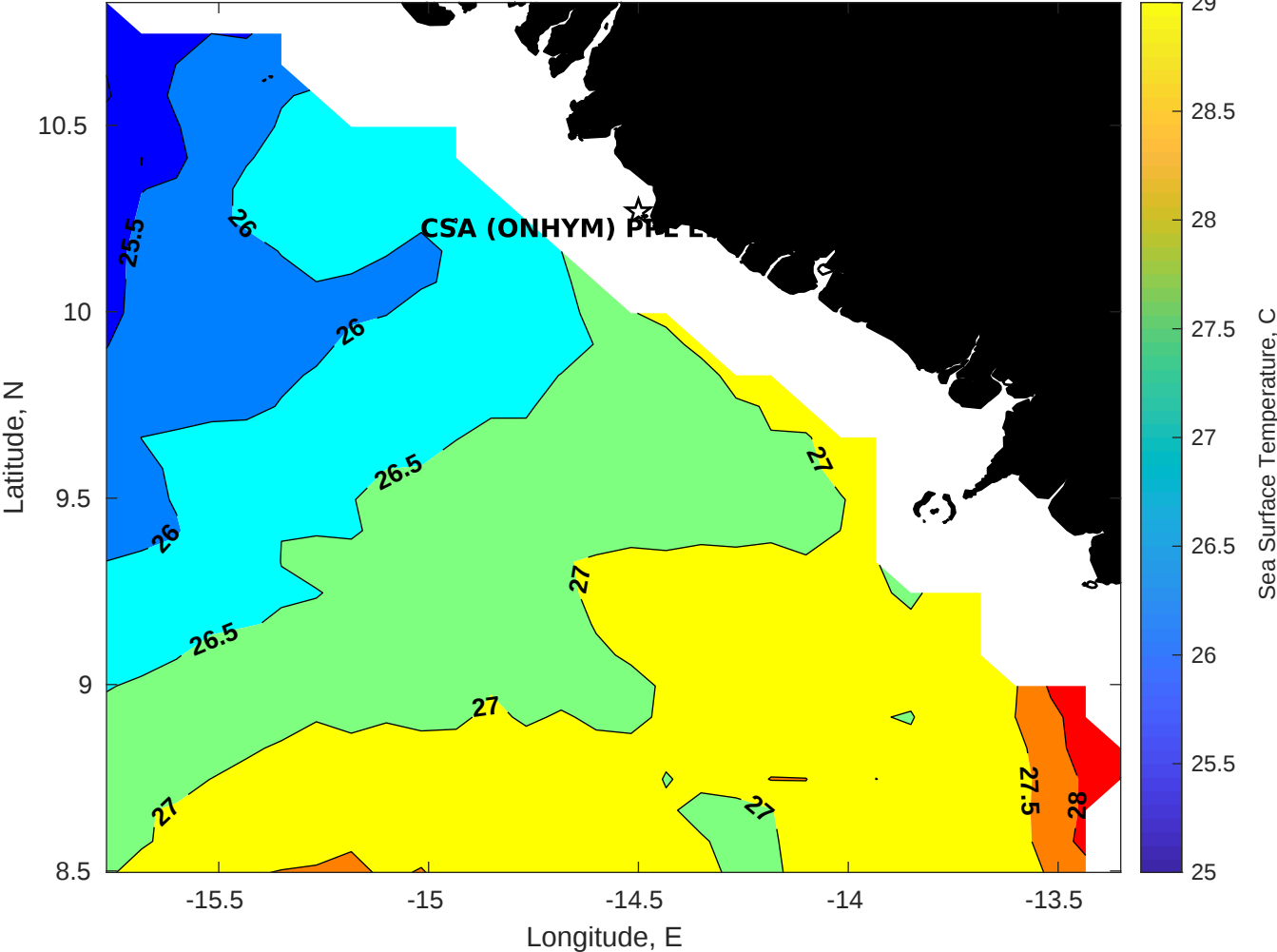
SST for CSA (ONHYM) PPL EBS - Guinea at 21-Jan-2026 00:00:00
