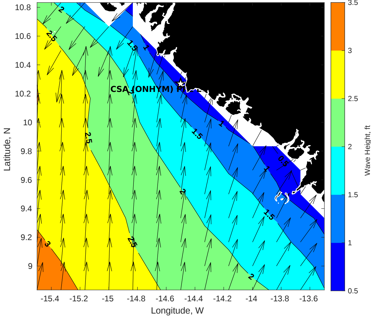
GFS Wave Height (ft) for CSA (ONHYM) PPL EBS - Guinea at 22-Jan-2026 09:00:00
