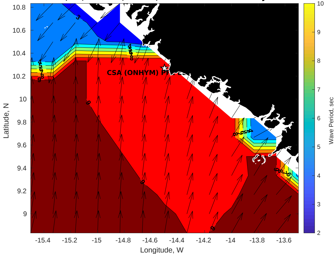
GFS Wave Period (sec) for CSA (ONHYM) PPL EBS - Guinea at 22-Jan-2026 09:00:00
