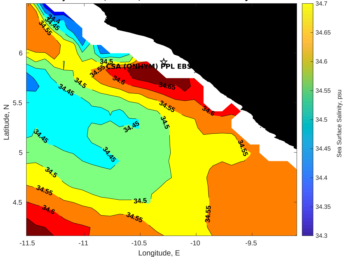
Surface Salinity for CSA (ONHYM) PPL EBS - Liberia at 21-Jan-2026 00:00:00
