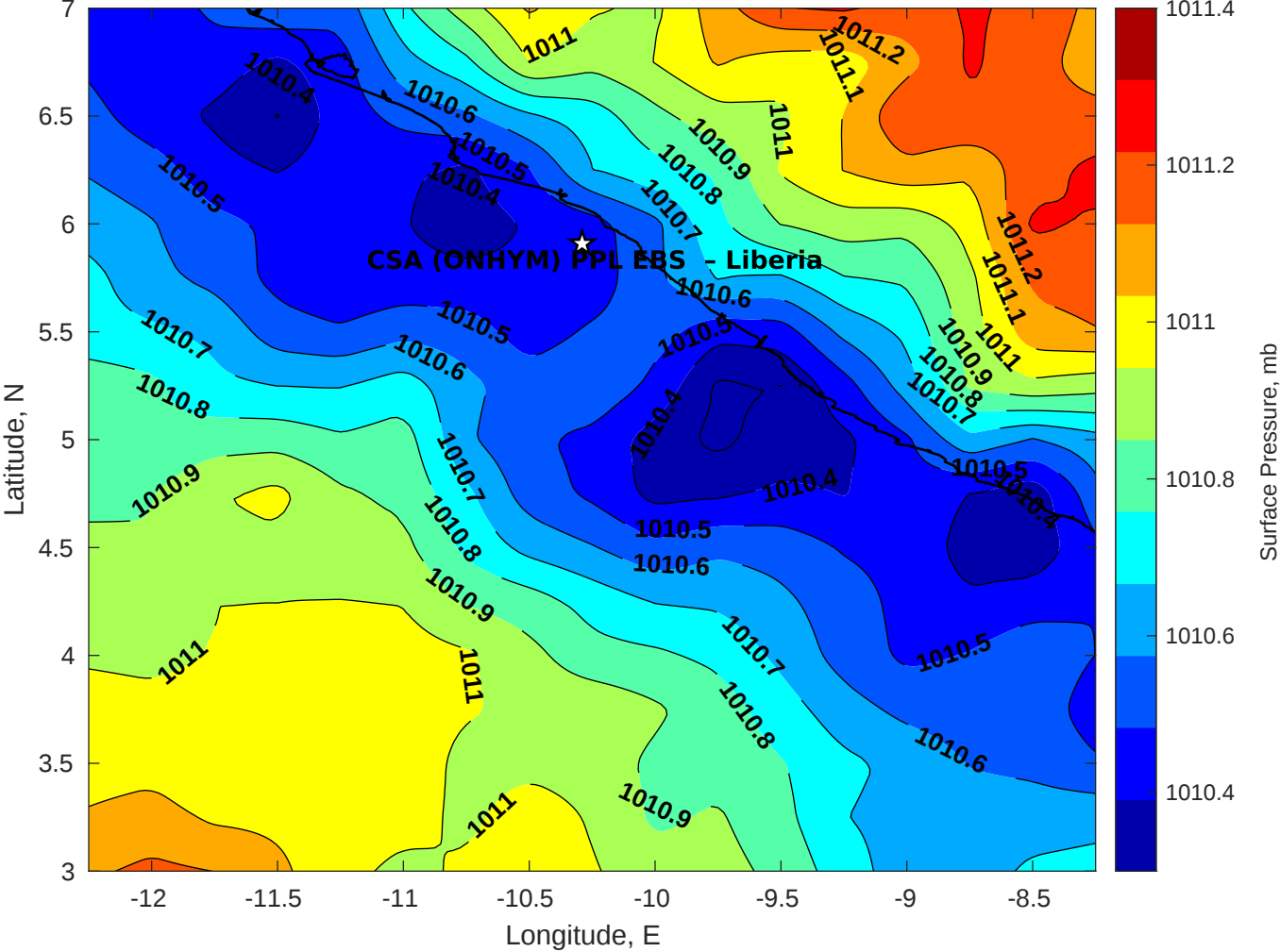
Surface Pressure (mb) for CSA (ONHYM) PPL EBS - Liberia at 22-Jan-2026 00:00:00
