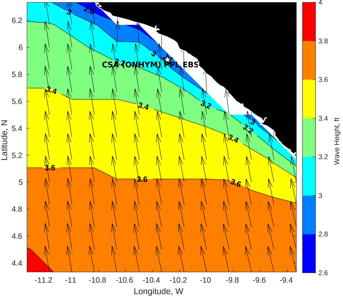
GFS Wave Height (ft) for CSA (ONHYM) PPL EBS - Liberia at 22-Jan-2026 09:00:00
