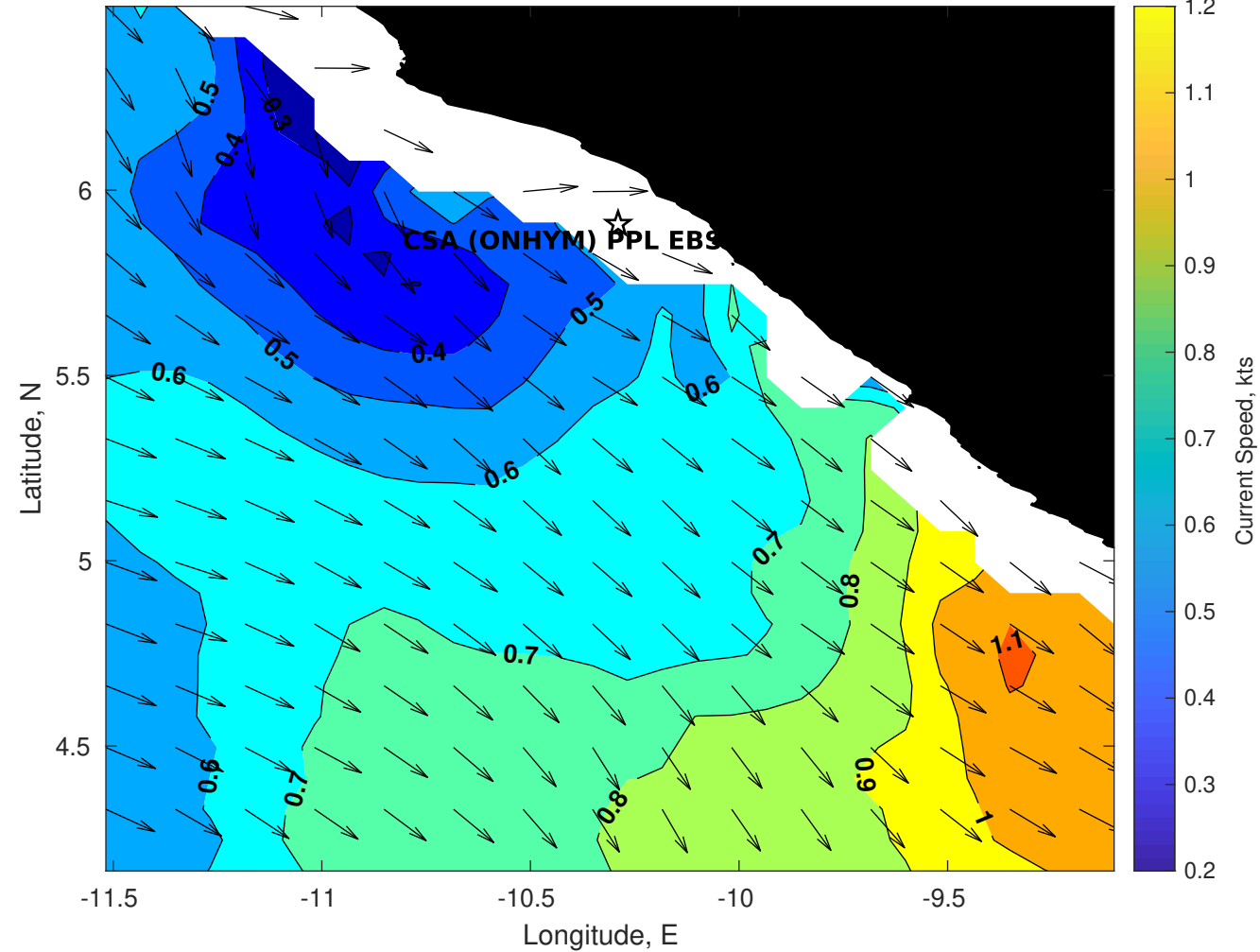
Surface Currents for CSA (ONHYM) PPL EBS - Liberia at 21-Jan-2026 00:00:00
