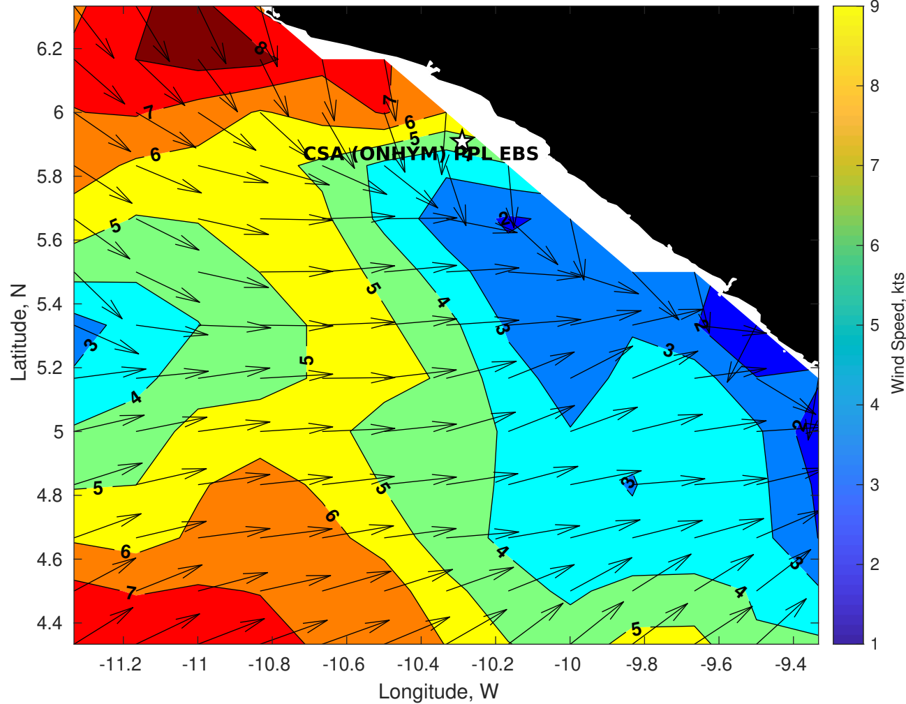
GFS Winds (kts) for CSA (ONHYM) PPL EBS - Liberia at 22-Jan-2026 09:00:00
