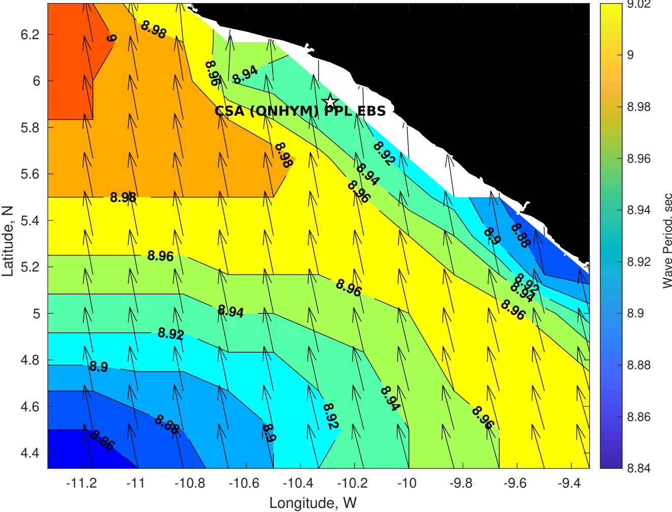
GFS Wave Period (sec) for CSA (QNHYM) PPL EBS - Liberia at 22-Jan-2026 09:00:00
