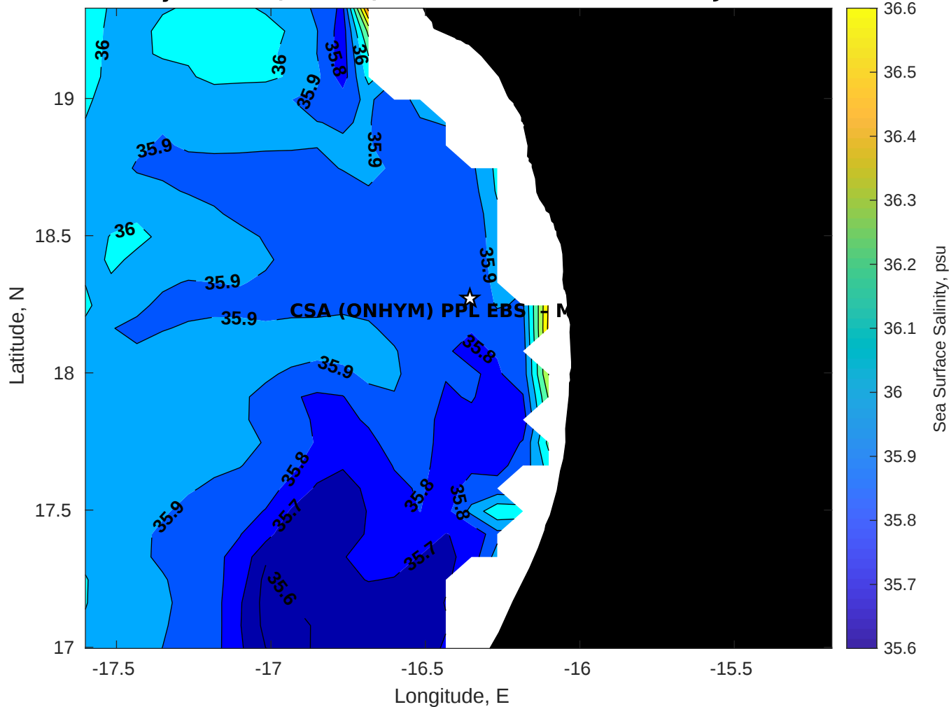
Surface Salinity for CSA (ONHYM) PPL EBS - Mauritania at 21-Jan-2026 00:00:00
