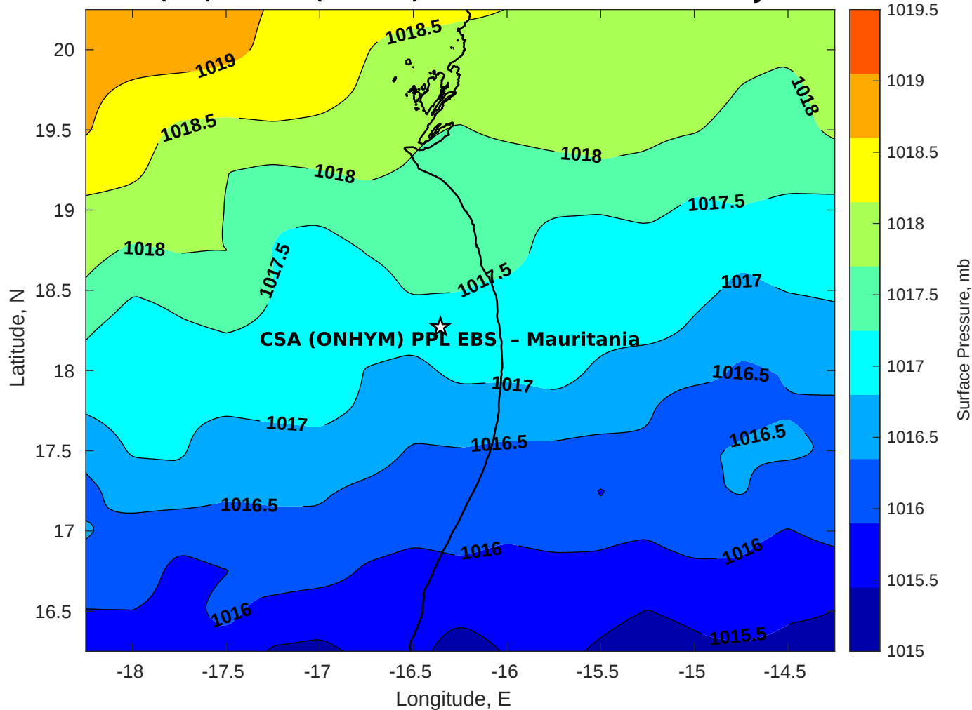
Surface Pressure (mb) for CSA (ONHYM) PPL EBS - Mauritania at 22-Jan-2026 00:00:00
