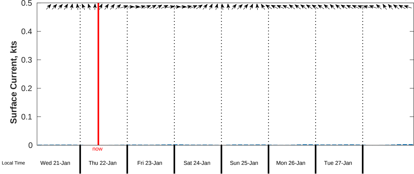
Surface Current Forecast for CSA (ONHYM) PPL EBS - Mauritania from 21-Jan-2026 00:00:00 to 29-Jan-2026 00:00:00
