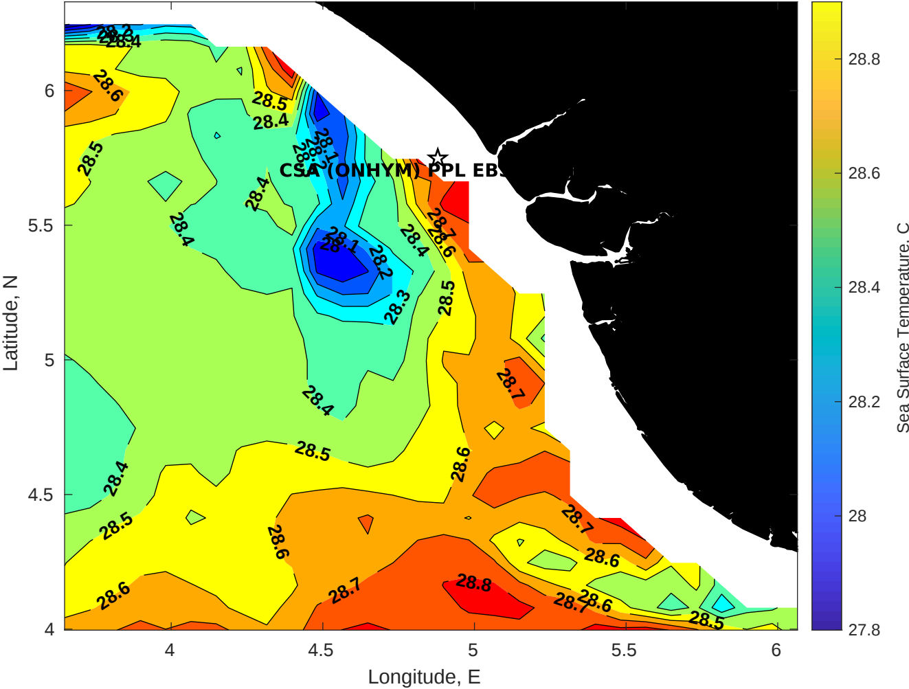
SST for CSA (ONHYM) PPL EBS - Nigeria at 21-Jan-2026 00:00:00
