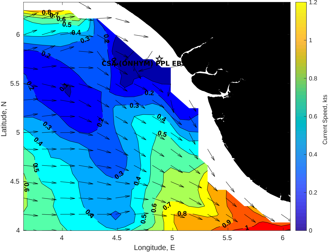
Surface Currents for CSA (ONHYM) PPL EBS - Nigeria at 21-Jan-2026 00:00:00
