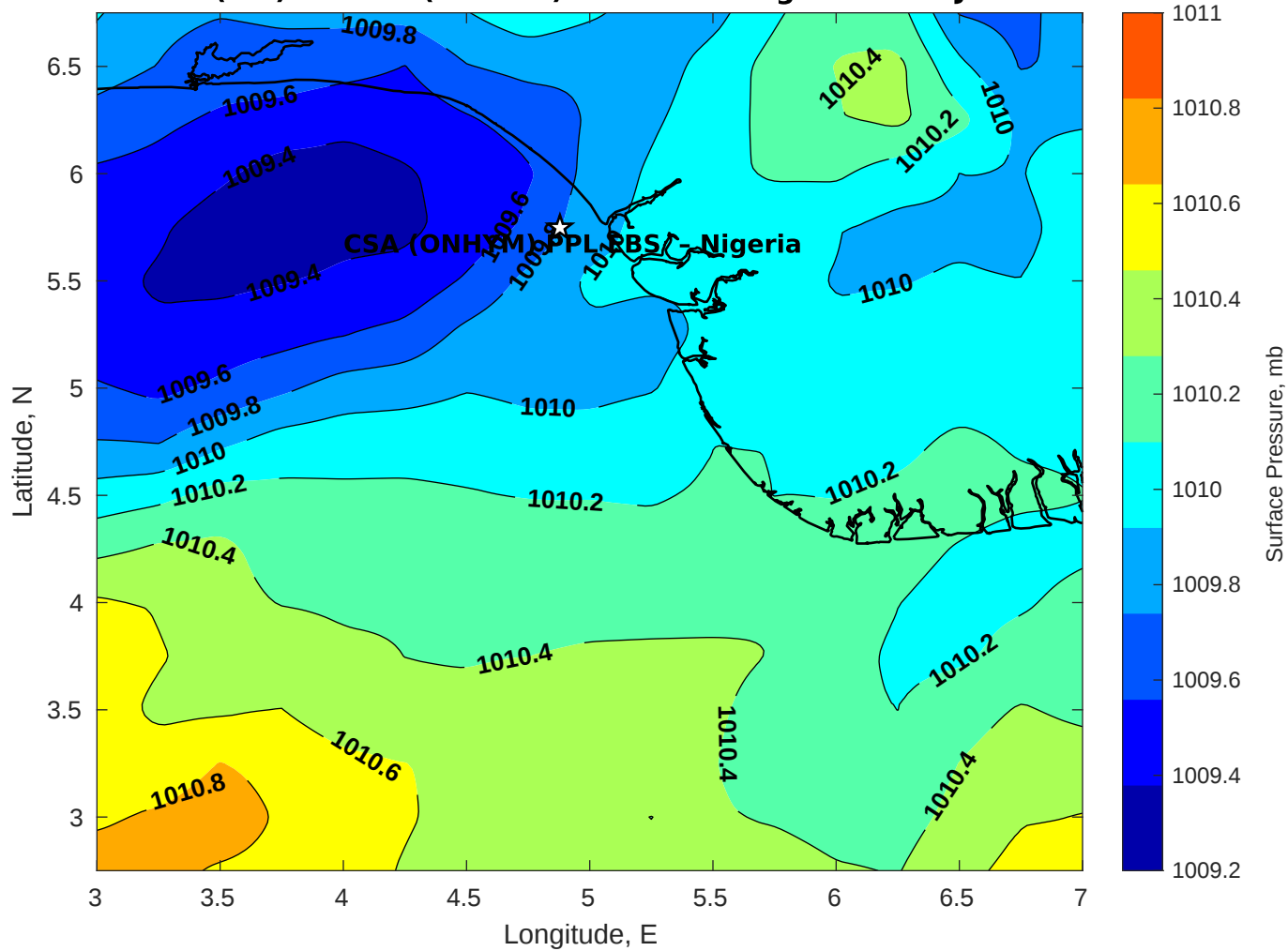
Surface Pressure (mb) for CSA (ONHYM) PPL EBS - Nigeria at 22-Jan-2026 00:00:00
