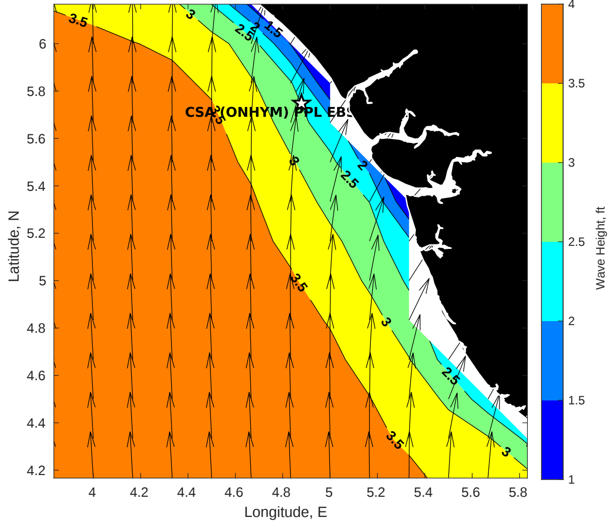
GFS Wave Height (ft) for CSA (ONHYM) PPL EBS - Nigeria at 22-Jan-2026 09:00:00
