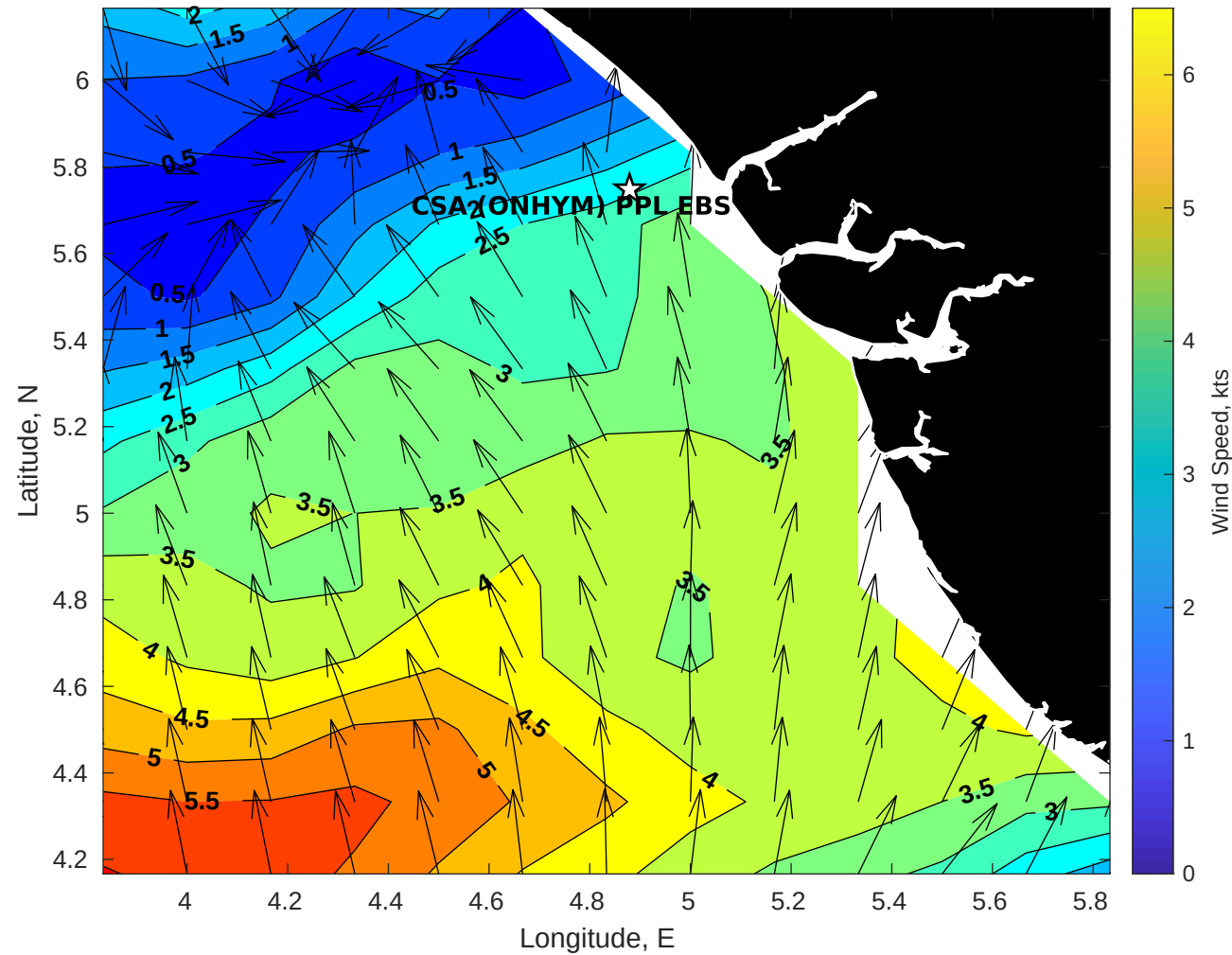
GFS Winds (kts) for CSA (ONHYM) PPL EBS - Nigeria at 22-Jan-2026 09:00:00
