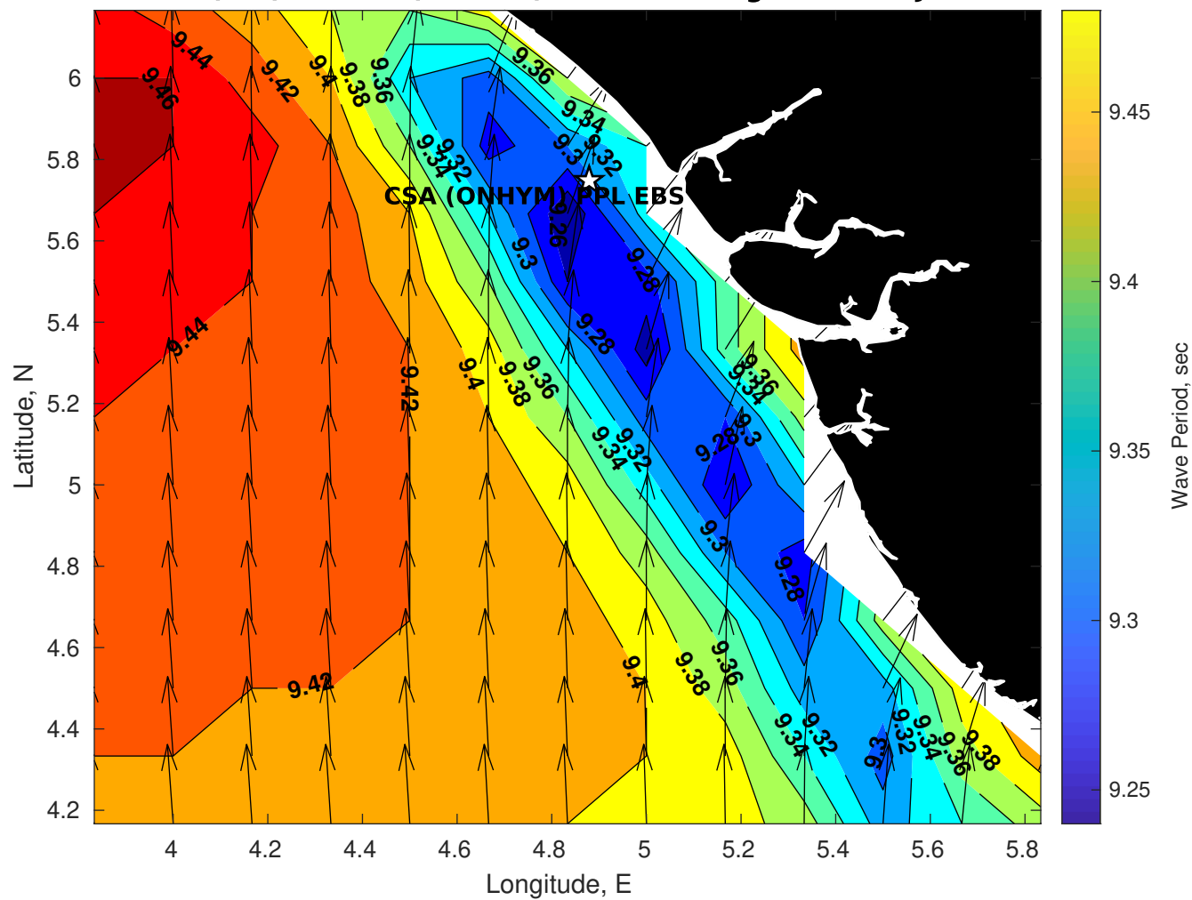
GFS Wave Period (sec) for CSA (ONHYM) PPL EBS - Nigeria at 22-Jan-2026 09:00:00
