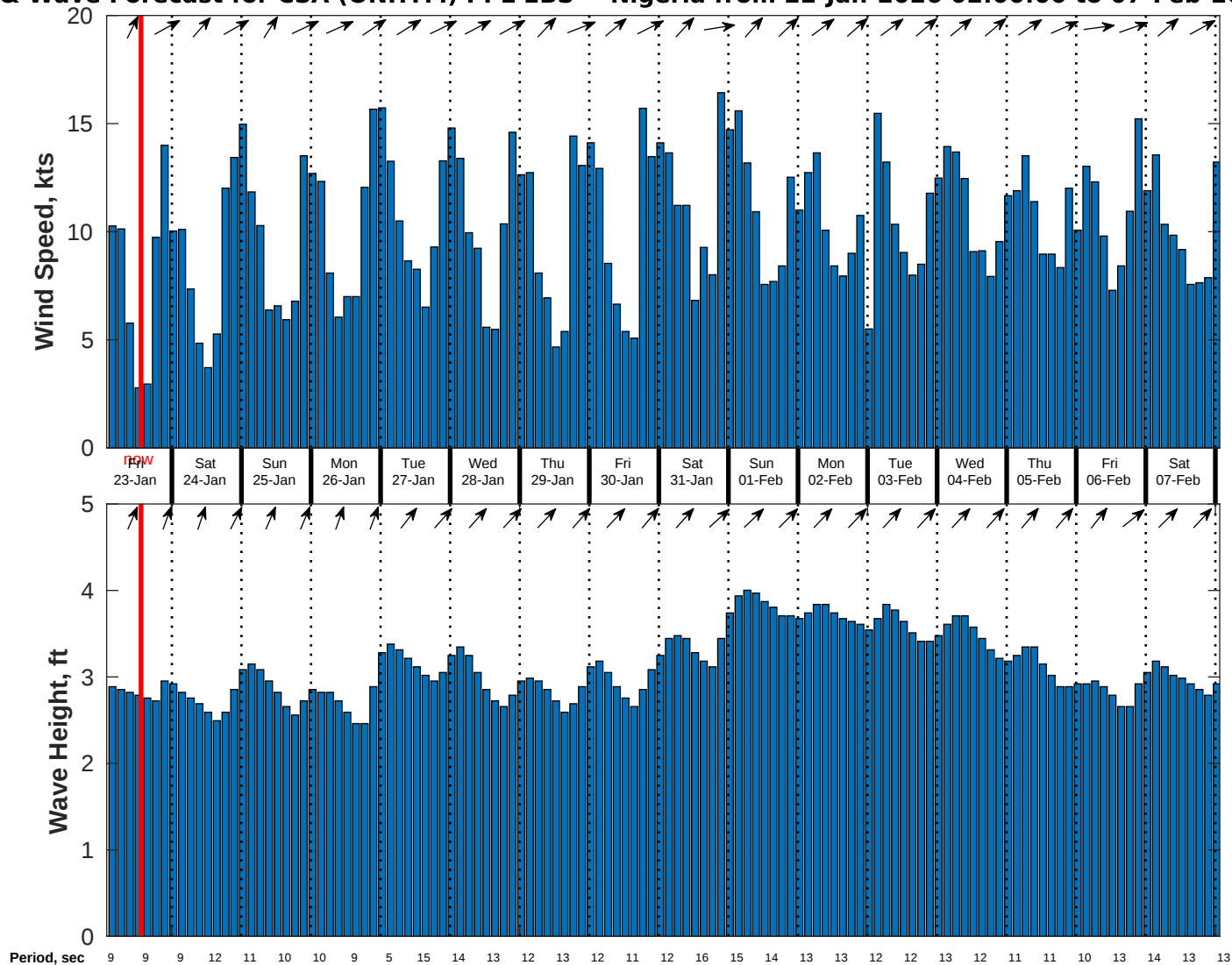
Wind & Wave Forecast for CSA (ONHYM) PPL EBS - Nigeria from 22-Jan-2026 02:00:00 to 07-Feb-2026 02:00:00
