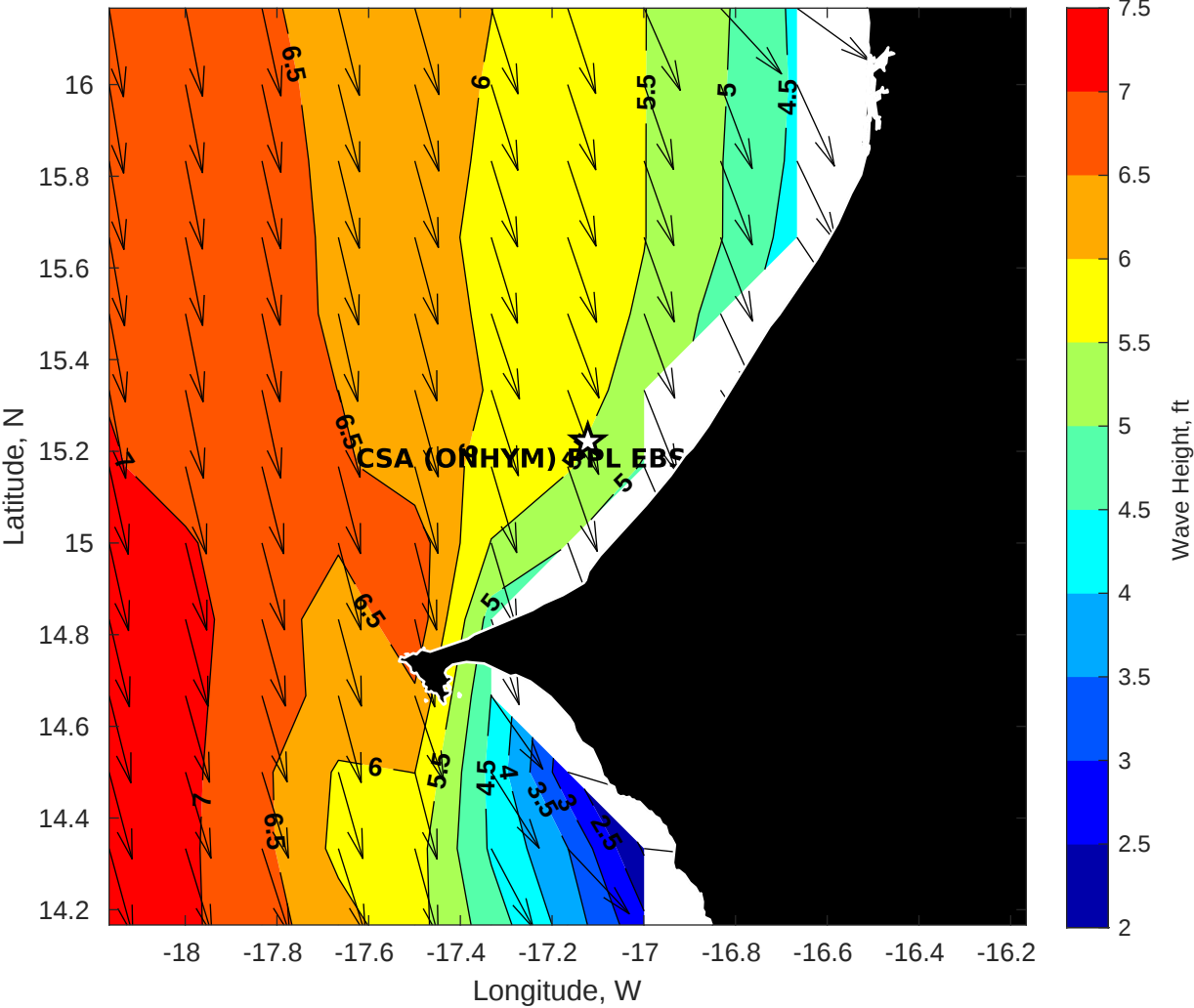
GFS Wave Height (ft) for CSA (ONHYM) PPL EBS - Senegal at 22-Jan-2026 09:00:00
