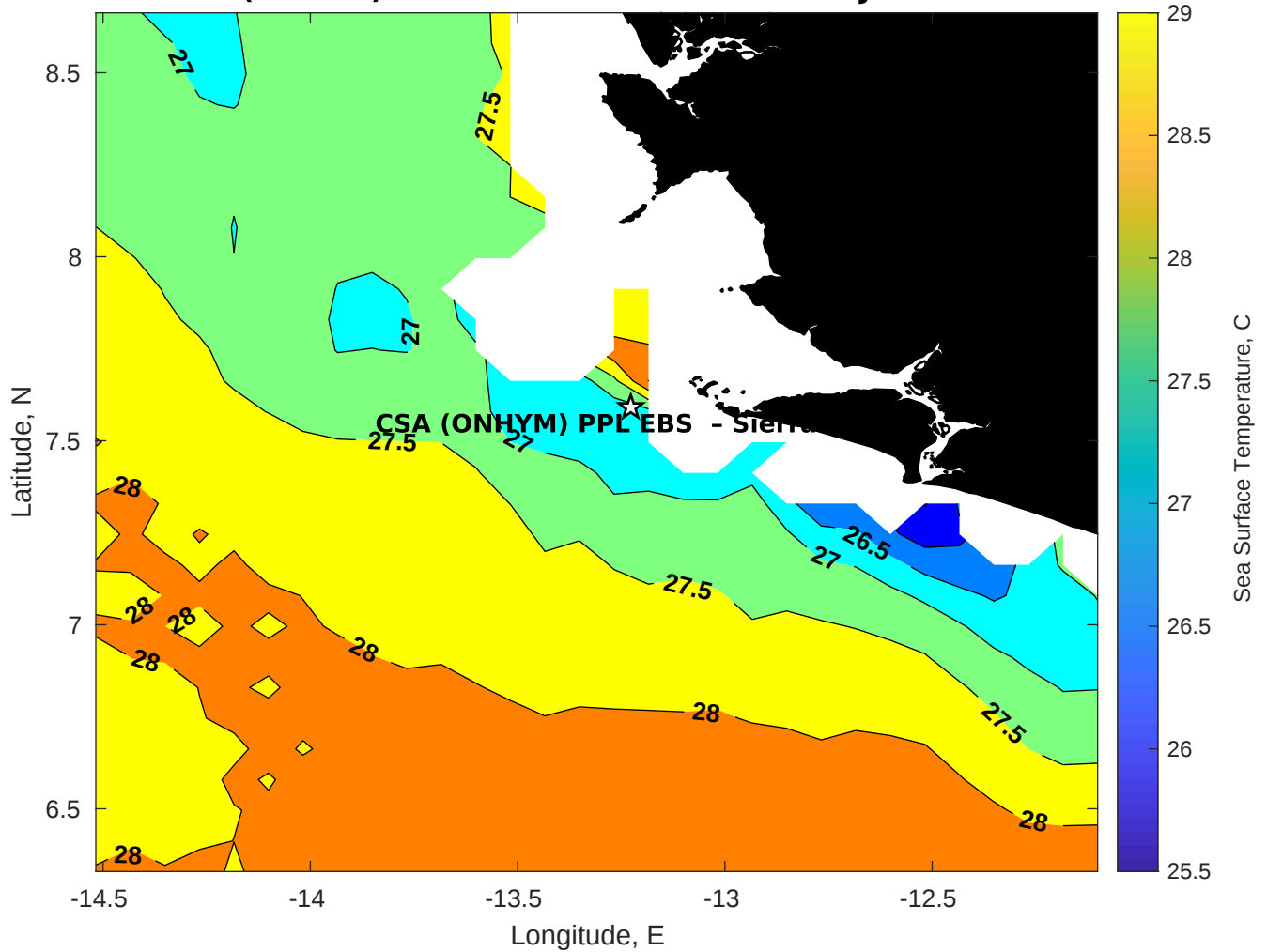
SST for CSA (ONHYM) PPL EBS - Sierra Leone at 21-Jan-2026 00:00:00
