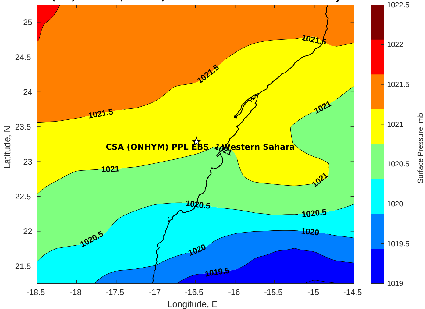
Surface Pressure (mb) for CSA (ONHYM) PPL EBS - Western Sahara at 22-Jan-2026 00:00:00
