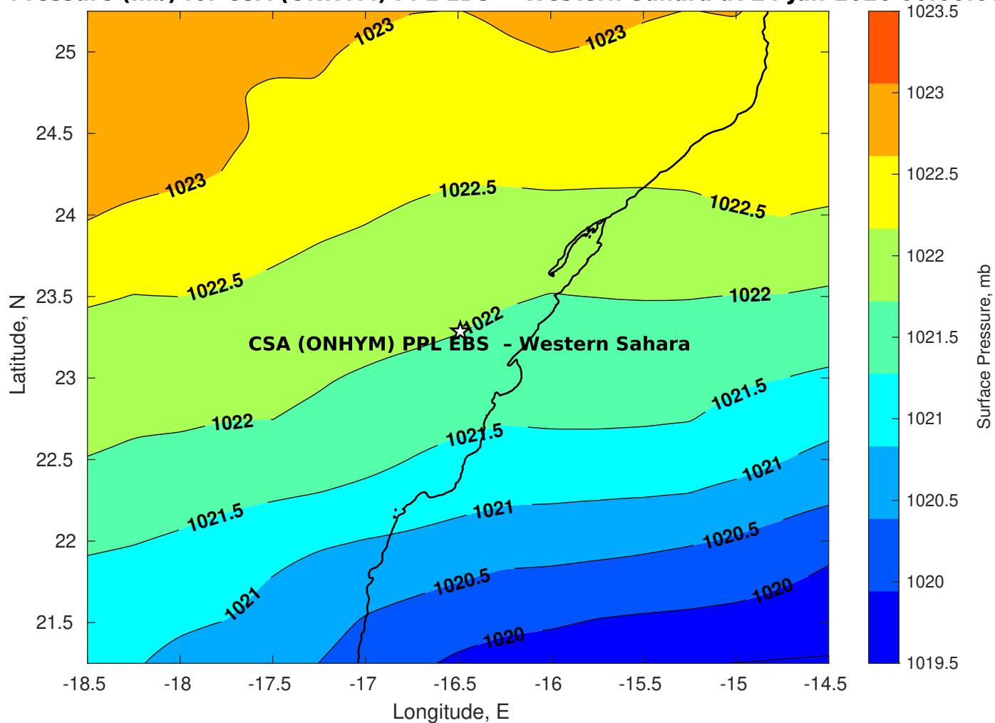
Surface Pressure (mb) for CSA (ONHYM) PPL EBS - Western Sahara at 24-Jan-2026 00:00:00
