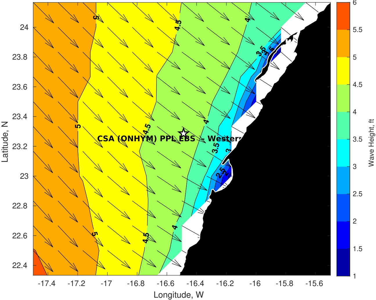
GFS Wave Height (ft) for CSA (ONHYM) PPL EBS - Western Sahara at 22-Jan-2026 09:00:00
