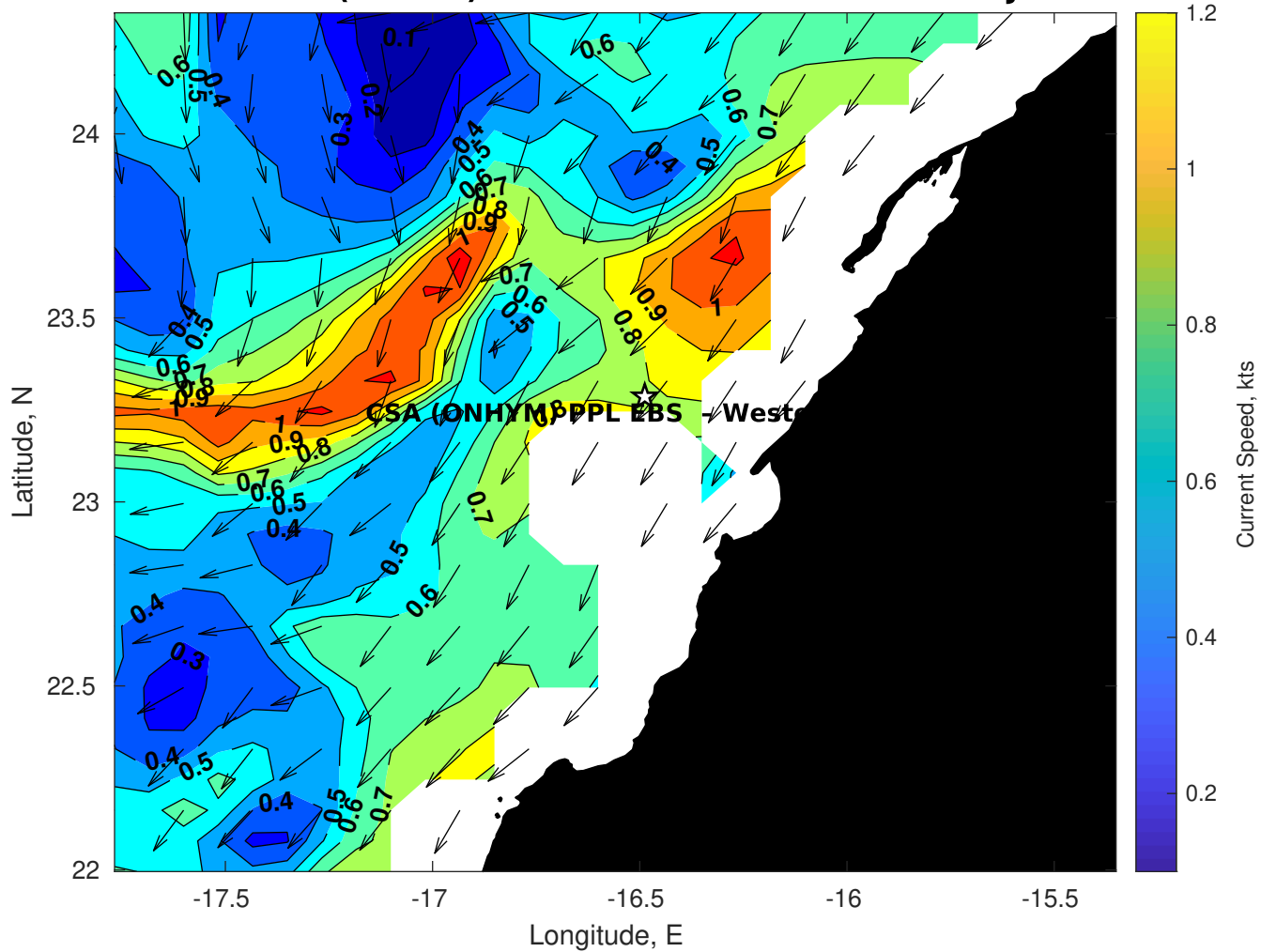
Surface Currents for CSA (ONHYM) PPL EBS - Western Sahara at 21-Jan-2026 00:00:00
