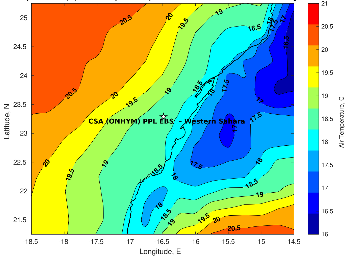
Air Temperature (C) for CSA (ONHYM) PPL EBS - Western Sahara at 22-Jan-2026
