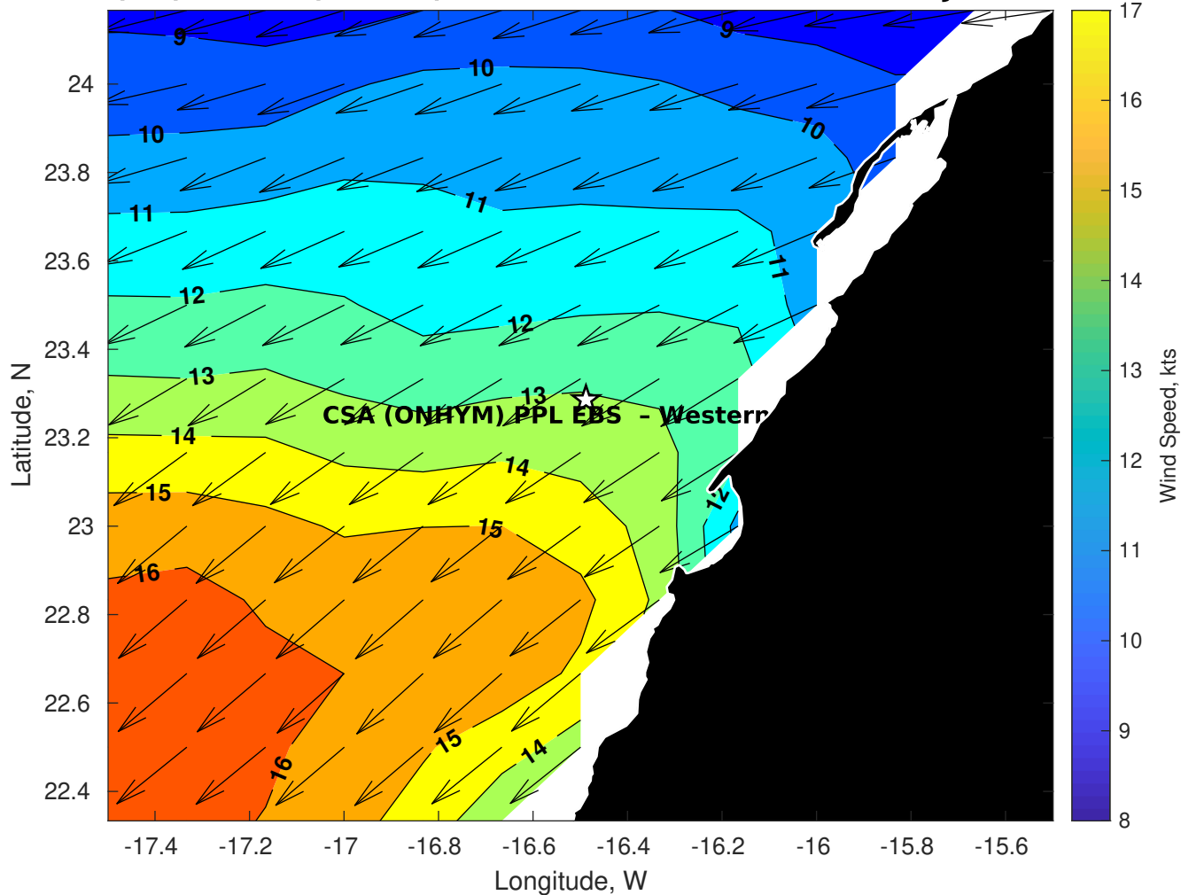
GFS Winds (kts) for CSA (ONHYM) PPL EBS - Western Sahara at 22-Jan-2026 09:00:00
