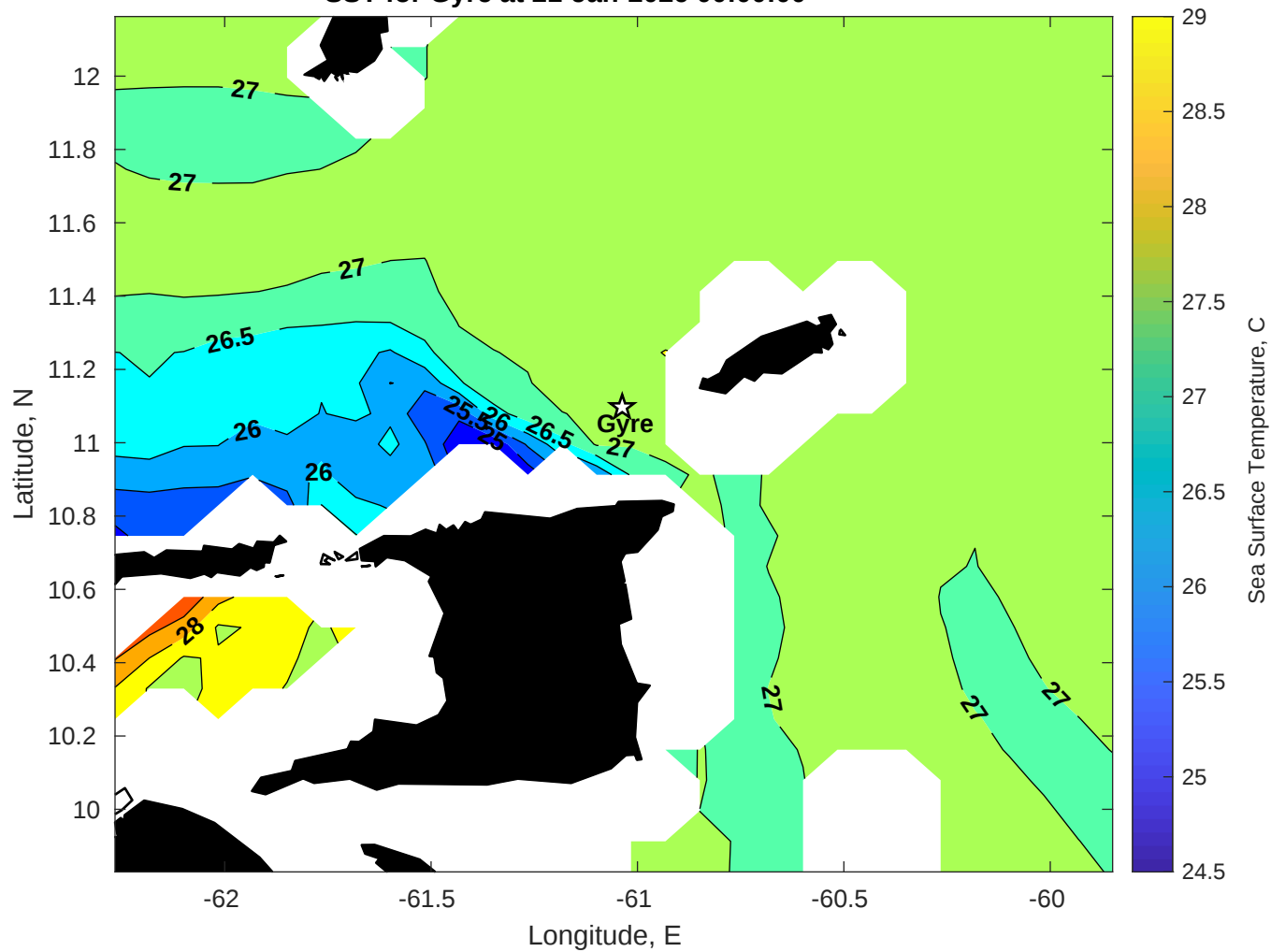
SST for Gyre at 21-Jan-2026 00:00:00
