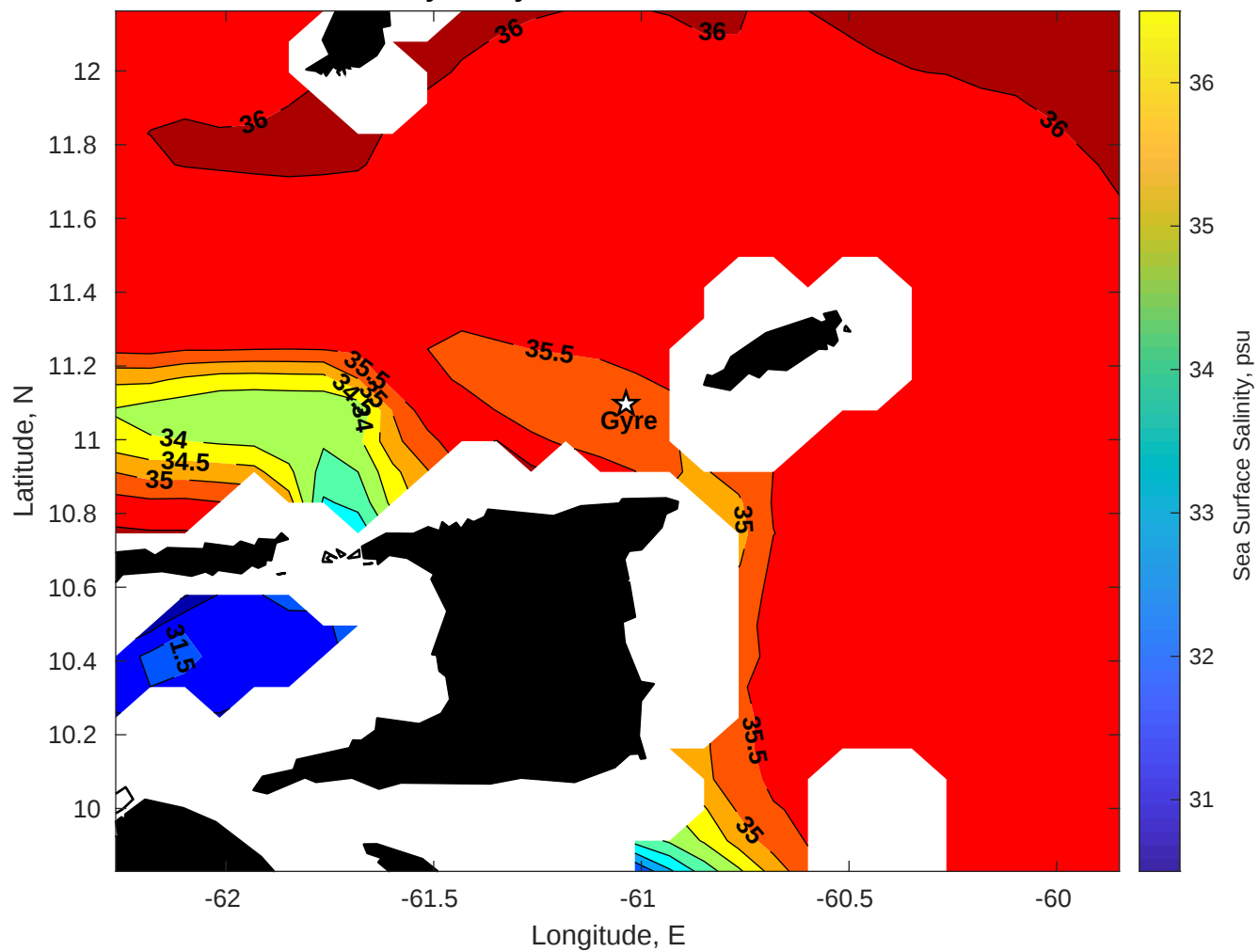
Surface Salinity for Gyre at 21-Jan-2026 00:00:00
