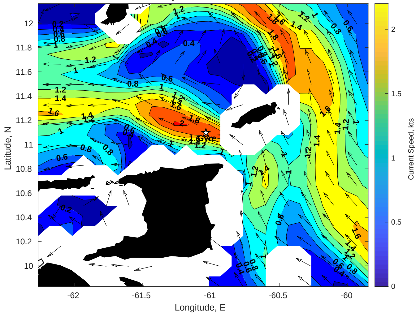
Surface Currents for Gyre at 21-Jan-2026 00:00:00
