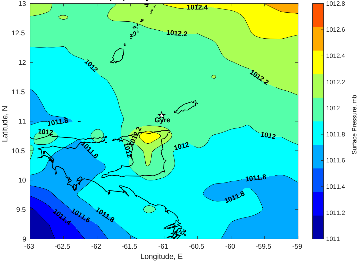
Surface Pressure (mb) for Gyre at 22-Jan-2026 00:00:00
