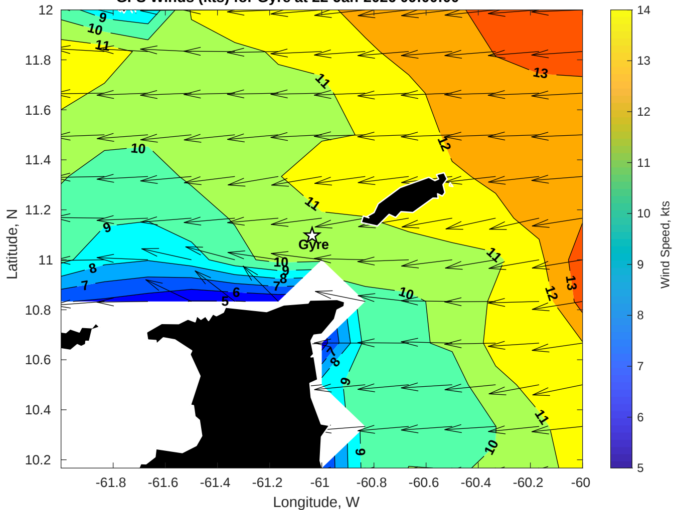
GFS Winds (kts) for Gyre at 22-Jan-2026 09:00:00
