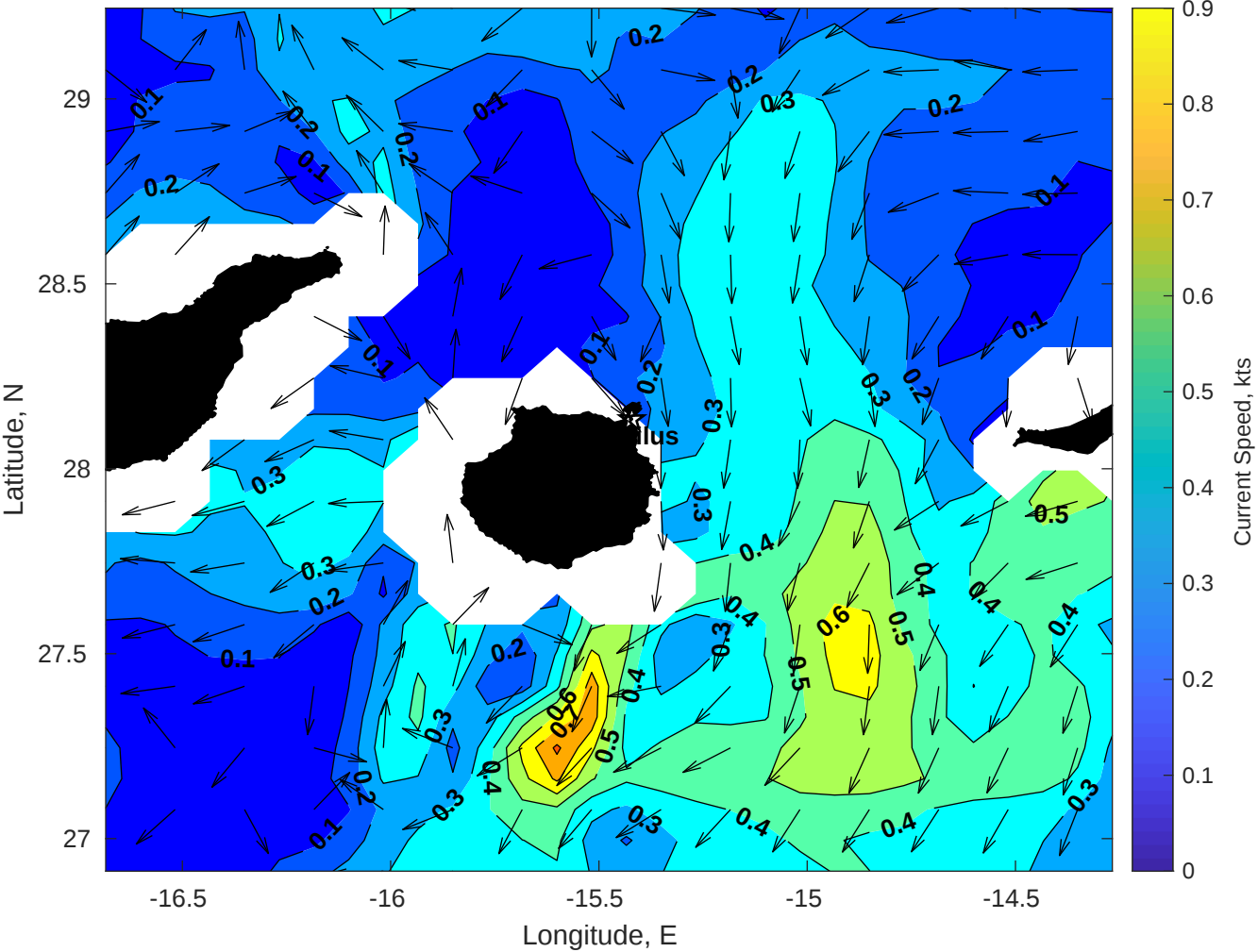
Surface Currents for Nautilus at 21-Jan-2026 00:00:00
