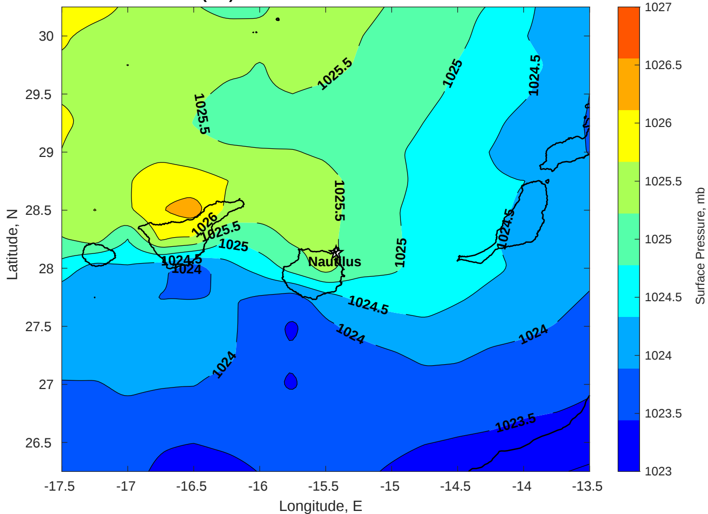
Surface Pressure (mb) for Nautilus at 24-Jan-2026 00:00:00
