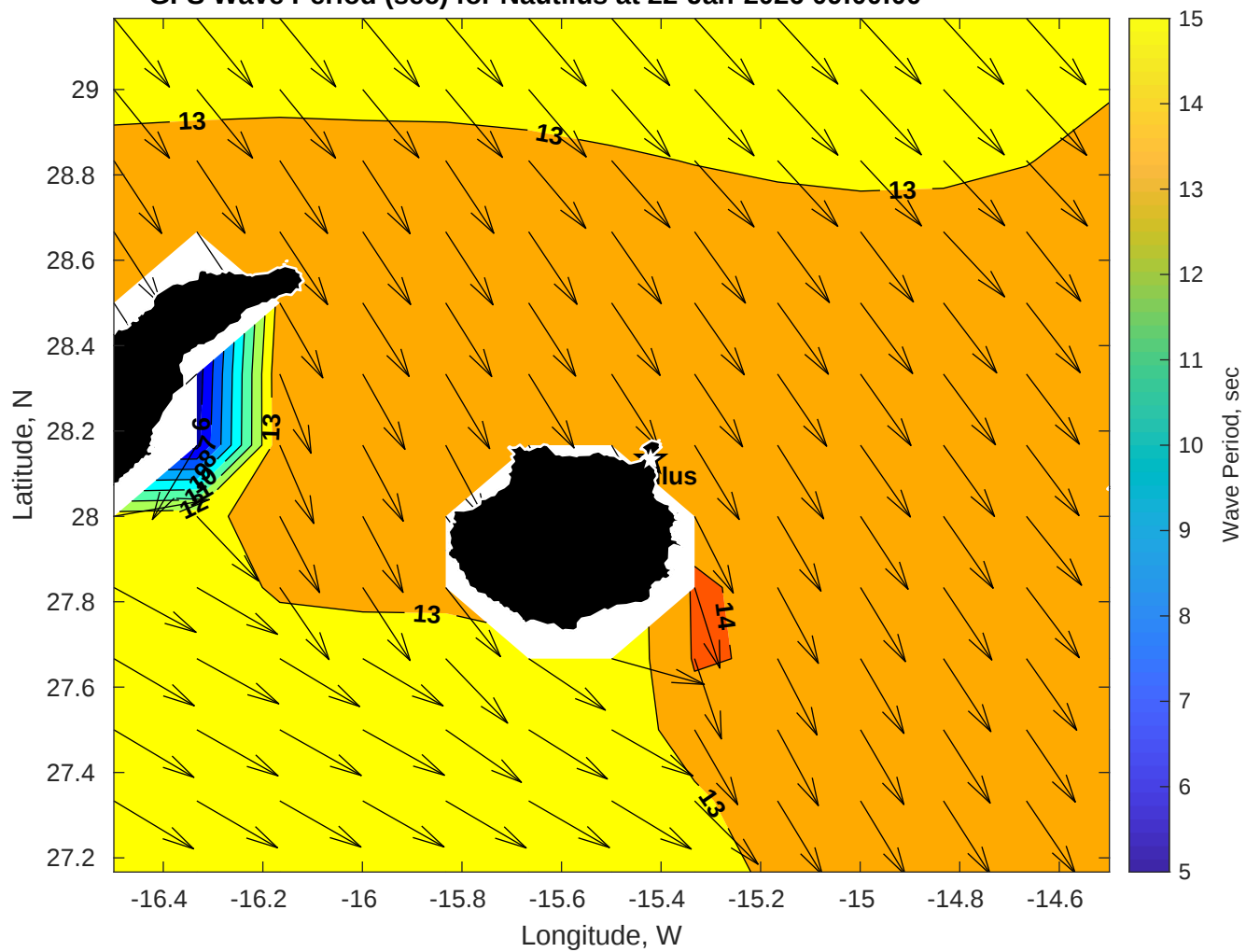
GFS Wave Period (sec) for Nautilus at 22-Jan-2026 09:00:00
