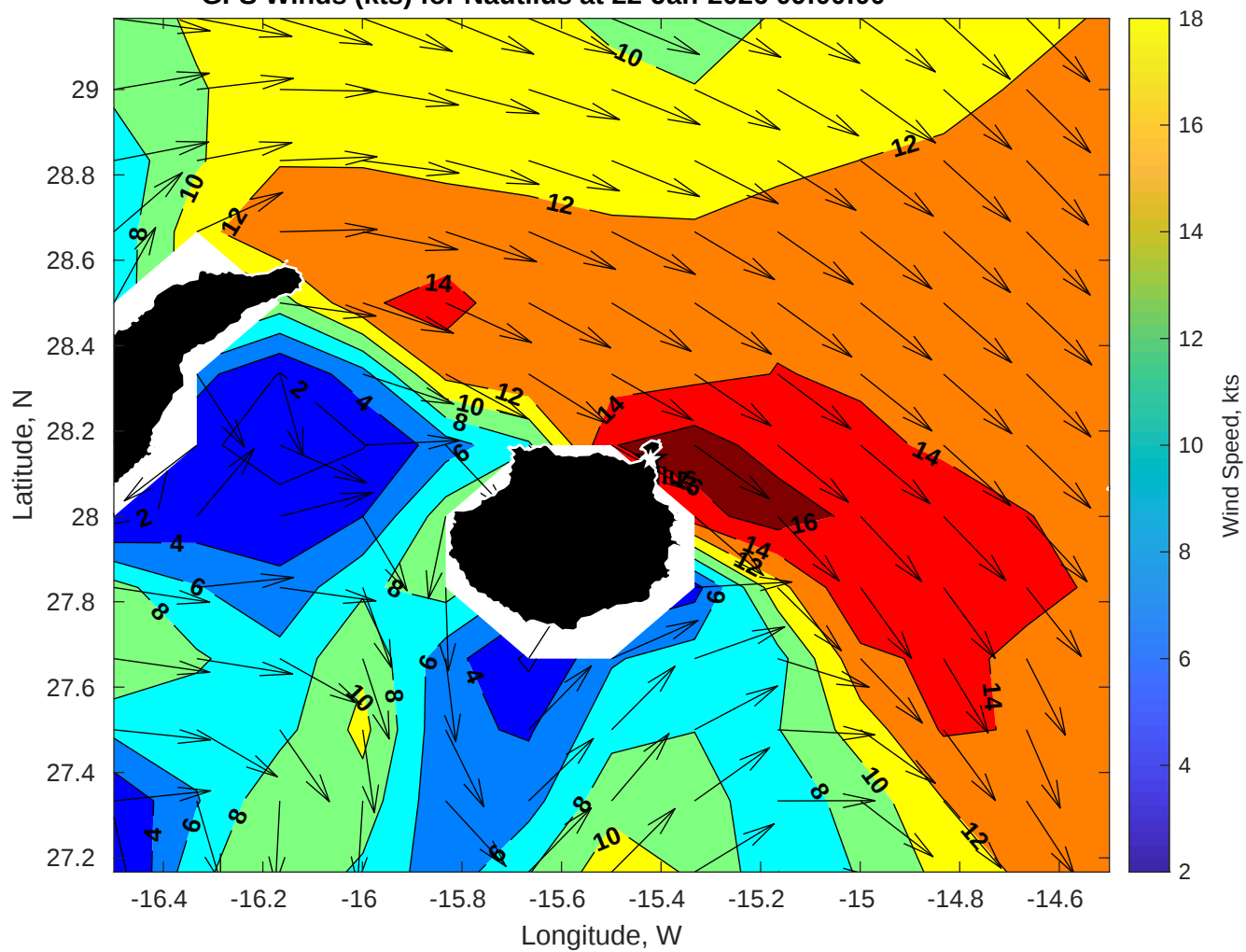
GFS Winds (kts) for Nautilus at 22-Jan-2026 09:00:00
