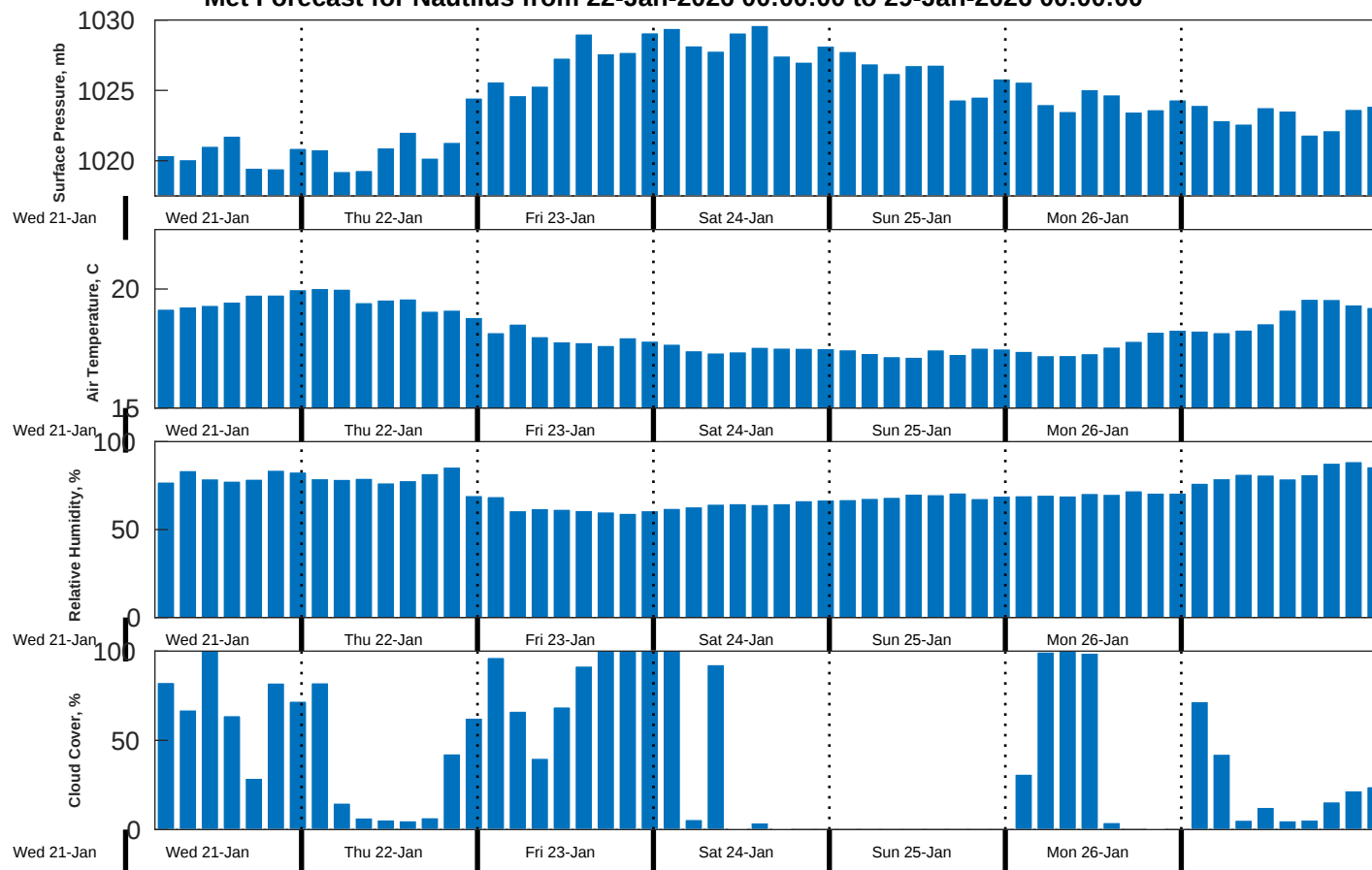
Met Forecast for Nautilus from 22-Jan-2026 00:00:00 to 29-Jan-2026 00:00:00
