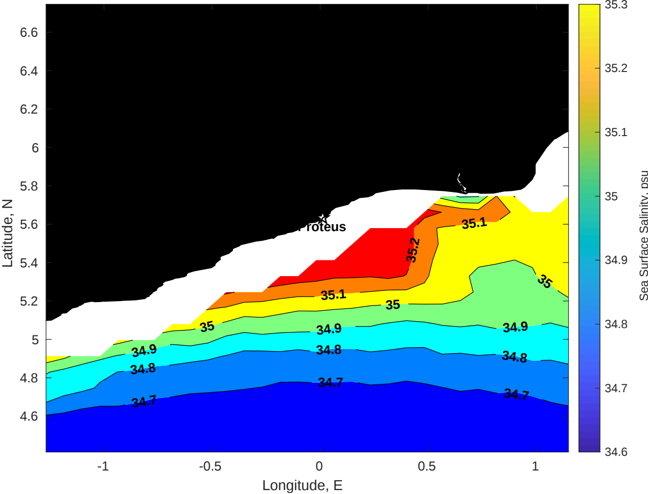
Surface Salinity for Proteus at 21-Jan-2026 00:00:00
