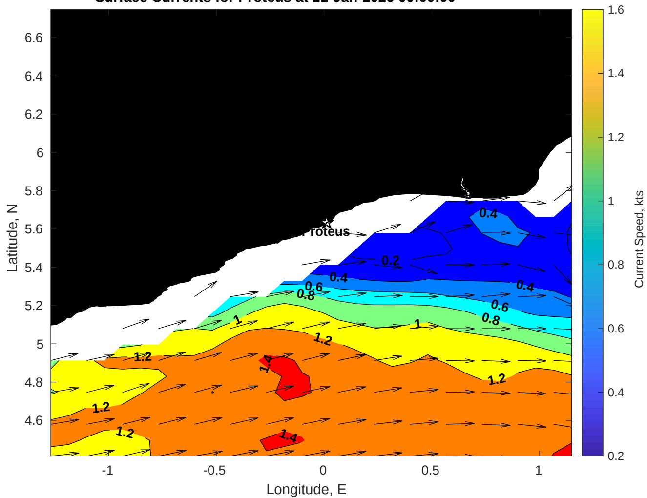
Surface Currents for Proteus at 21-Jan-2026 00:00:00
