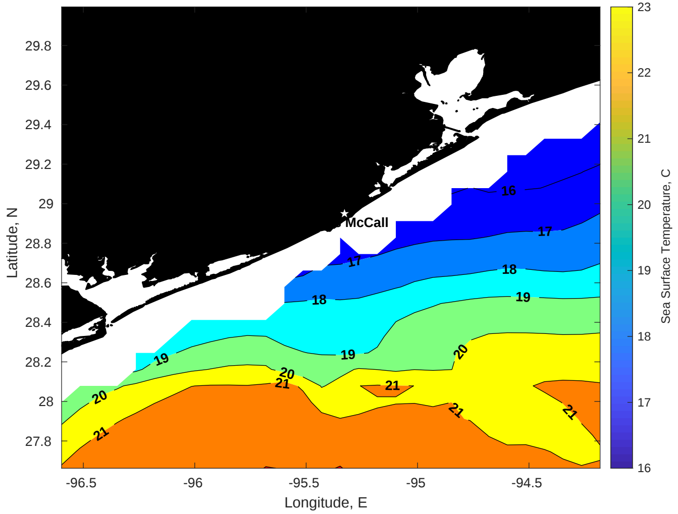
SST for Brooks McCall at 22-Jan-2026 00:00:00
