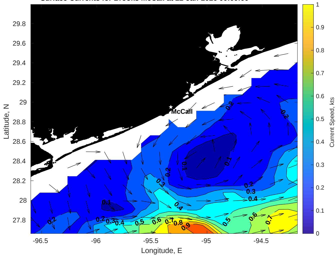
Surface Currents for Brooks McCall at 22-Jan-2026 00:00:00
