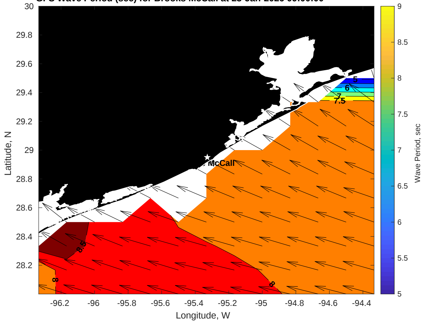
GFS Wave Period (sec) for Brooks McCall at 23-Jan-2026 09:00:00
