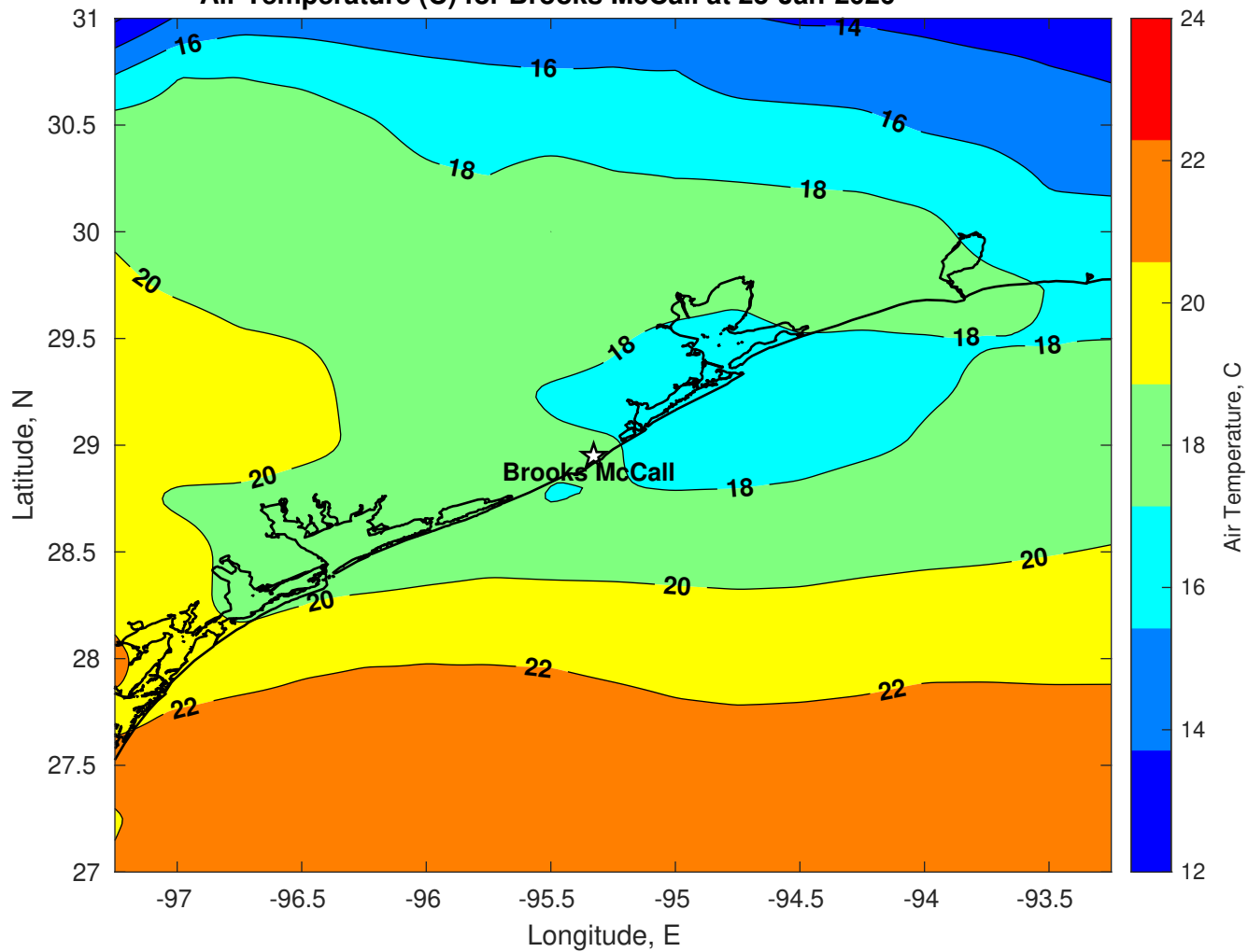
Air Temperature (C) for Brooks McCall at 23-Jan-2026
