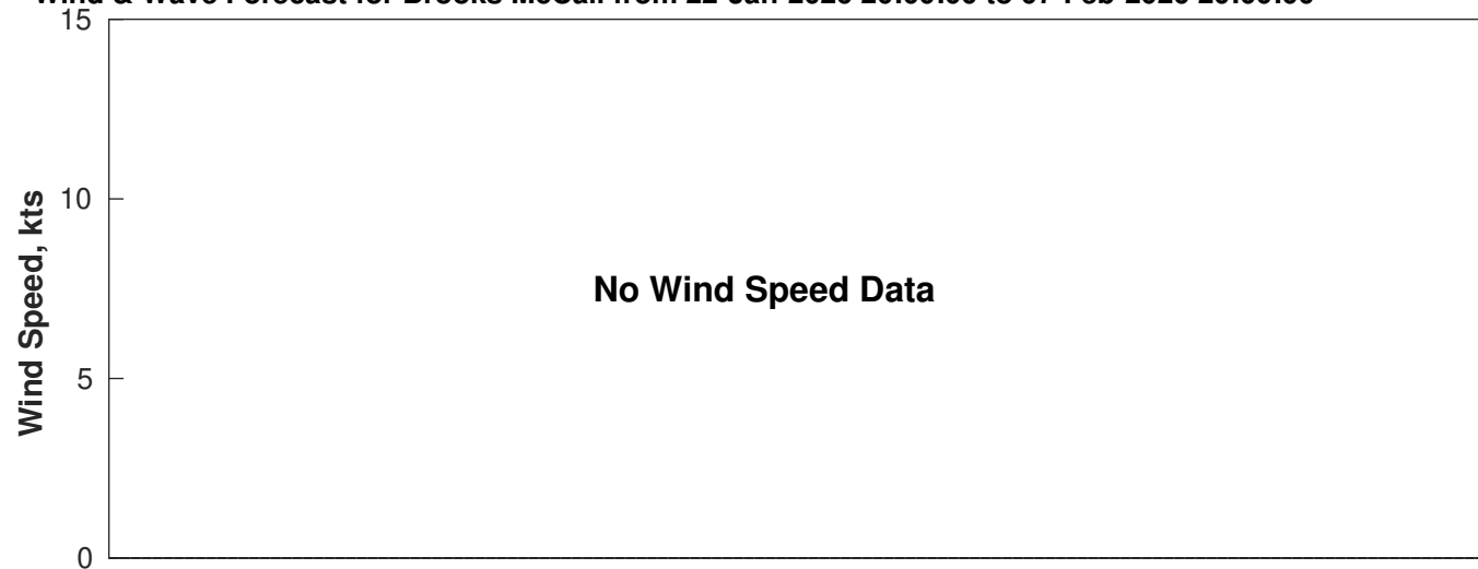
Wind & Wave Forecast for Brooks McCall from 22-Jan-2026 20:00:00 to 07-Feb-2026 20:00:00
