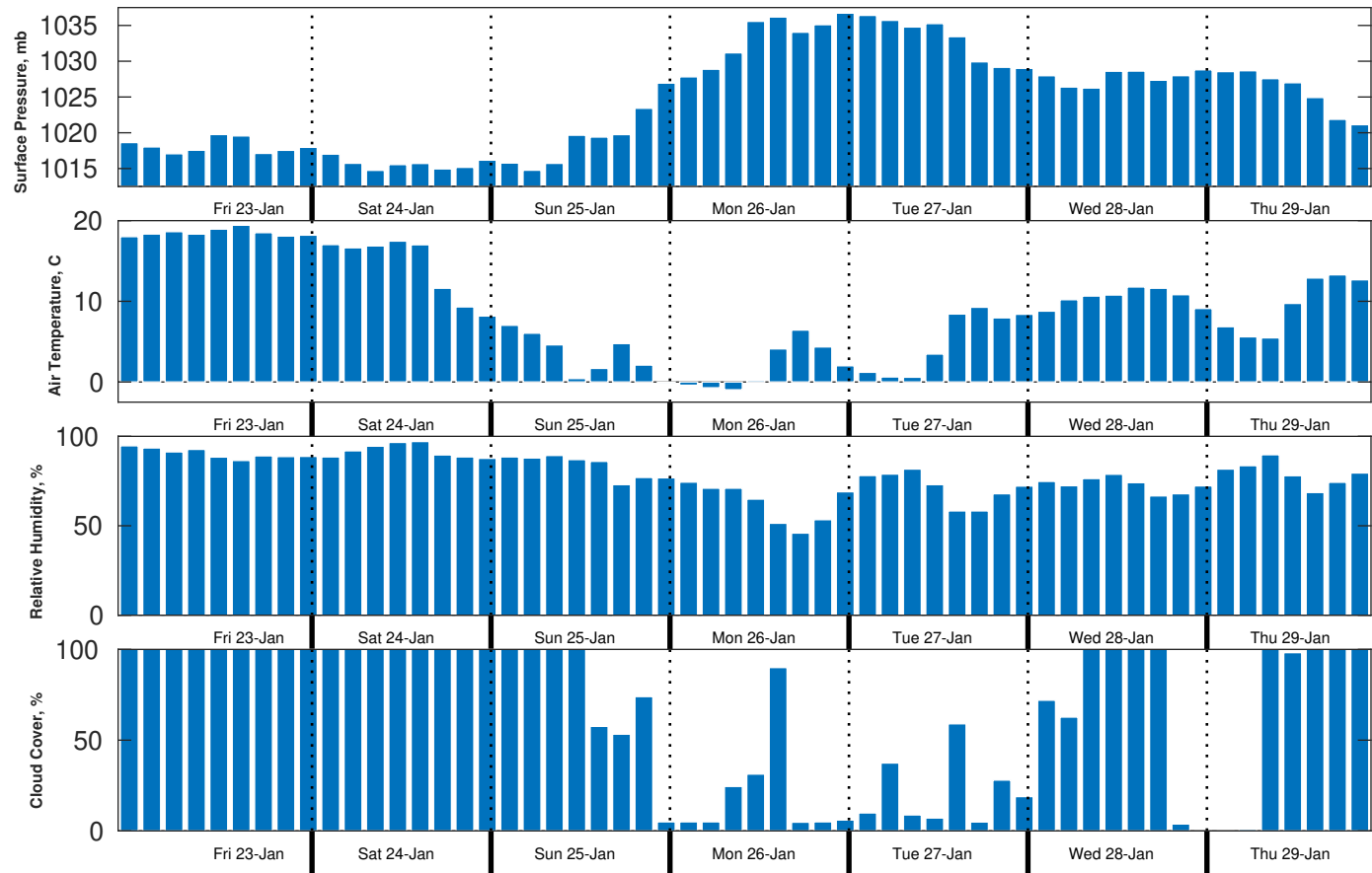
Met Forecast for Brooks McCall from 23-Jan-2026 00:00:00 to 30-Jan-2026 00:00:00
