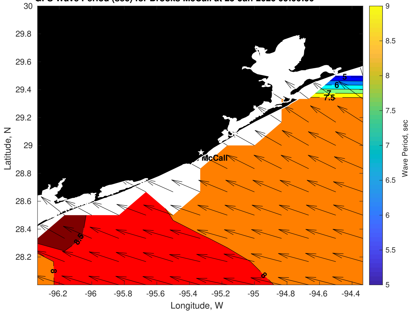
GFS Wave Period (sec) for Brooks McCall at 23-Jan-2026 09:00:00
