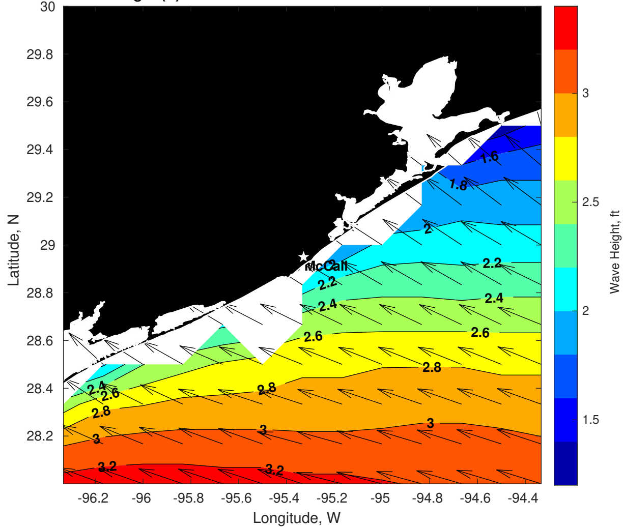
GFS Wave Height (ft) for Brooks McCall at 23-Jan-2026 09:00:00
