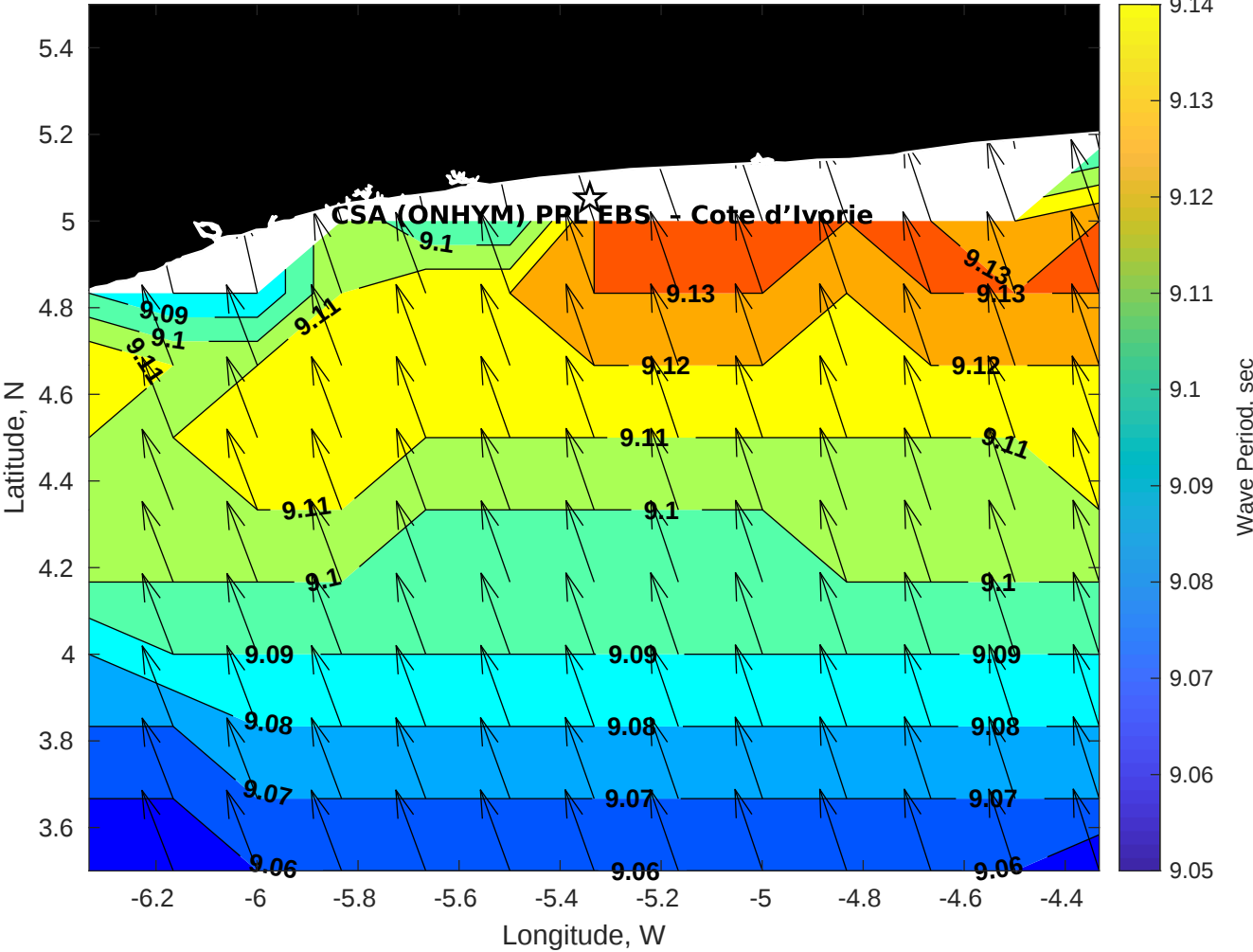
GFS Wave Period (sec) for CSA (ONHYM) PPL EBS - Cote d'Ivoire at 23-Jan-2026 09:00:00
