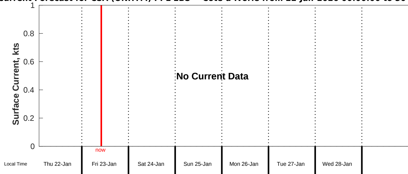
Surface Current Forecast for CSA (ONHYM) PPL EBS - Cote d'Ivoire from 22-Jan-2026 00:00:00 to 30-Jan-2026 00:00:00
