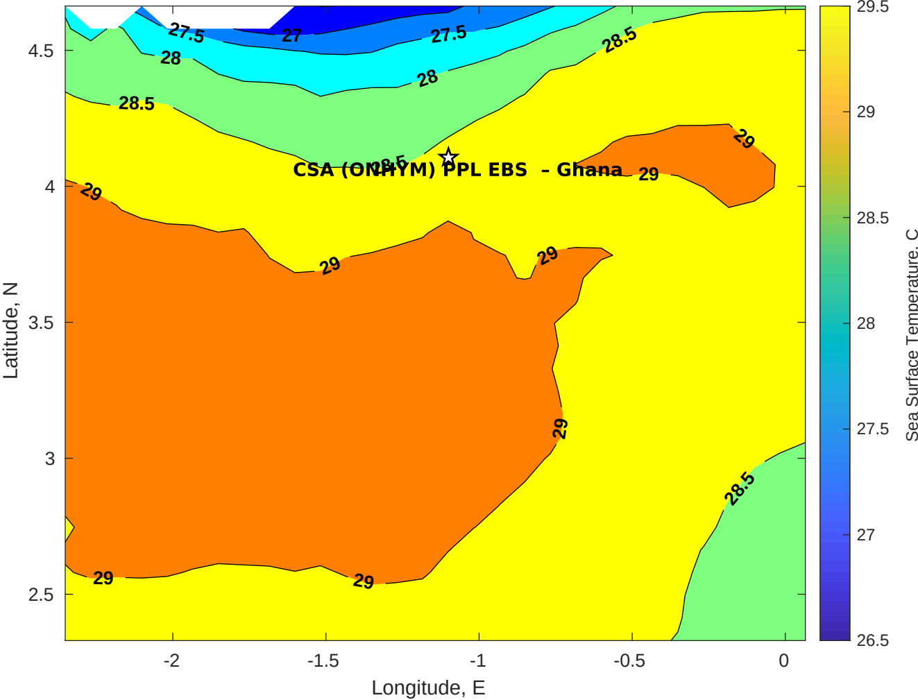
SST for CSA (ONHYM) PPL EBS - Ghana at 22-Jan-2026 00:00:00
