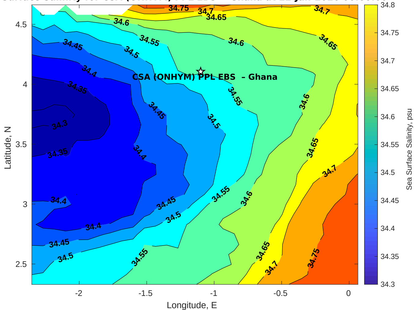
Surface Salinity for CSA (ONHYM) PPL EBS - Ghana at 22-Jan-2026 00:00:00
