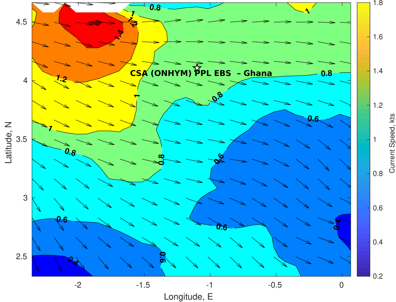
Surface Currents for CSA (ONHYM) PPL EBS - Ghana at 22-Jan-2026 00:00:00
