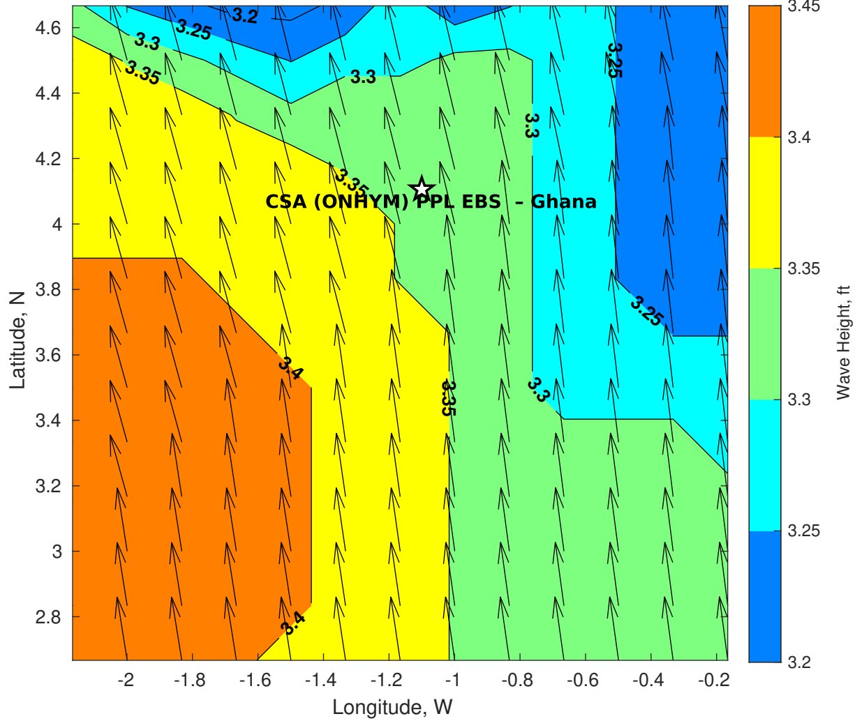
GFS Wave Height (ft) for CSA (ONHYM) PPL EBS - Ghana at 23-Jan-2026 09:00:00
