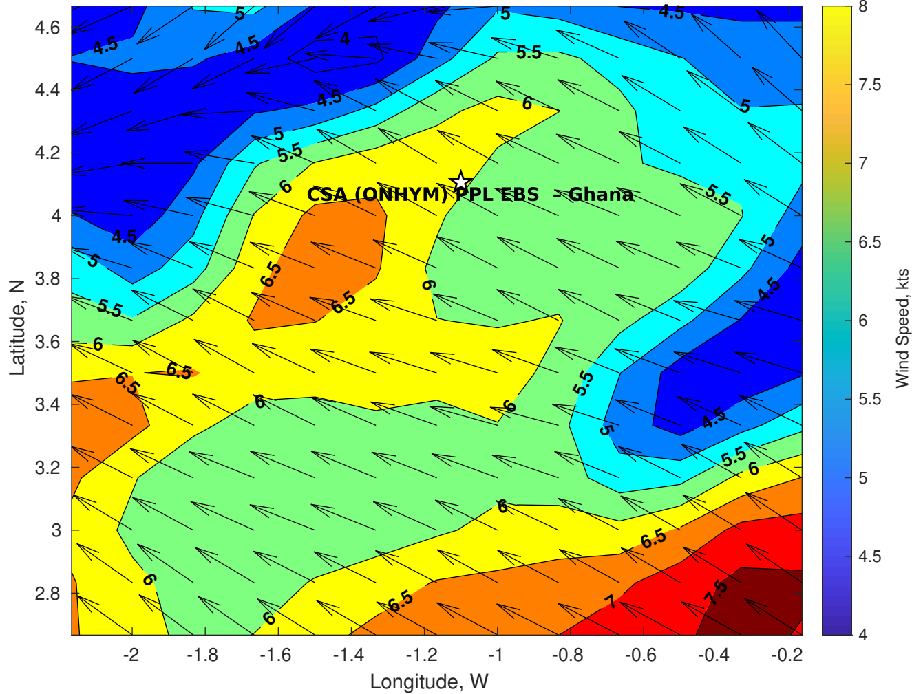
GFS Winds (kts) for CSA (ONHYM) PPL EBS - Ghana at 23-Jan-2026 09:00:00
