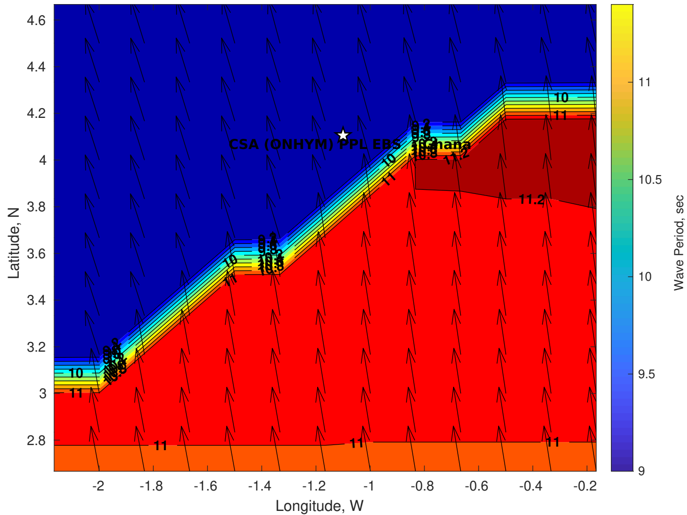
GFS Wave Period (sec) for CSA (ONHYM) PPL EBS - Ghana at 23-Jan-2026 09:00:00
