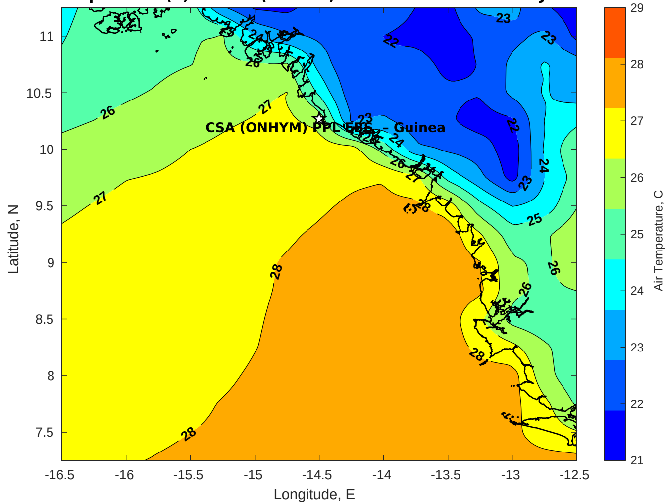
Air Temperature (C) for CSA (ONHYM) PPL EBS - Guinea at 23-Jan-2026
