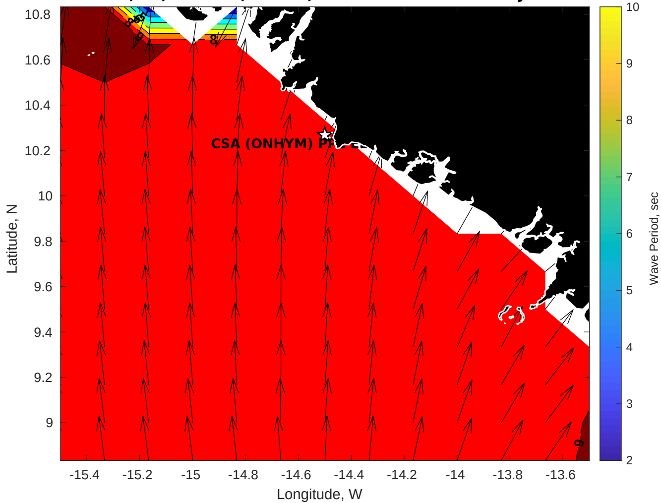
GFS Wave Period (sec) for CSA (ONHYM) PPL EBS - Guinea at 23-Jan-2026 09:00:00
