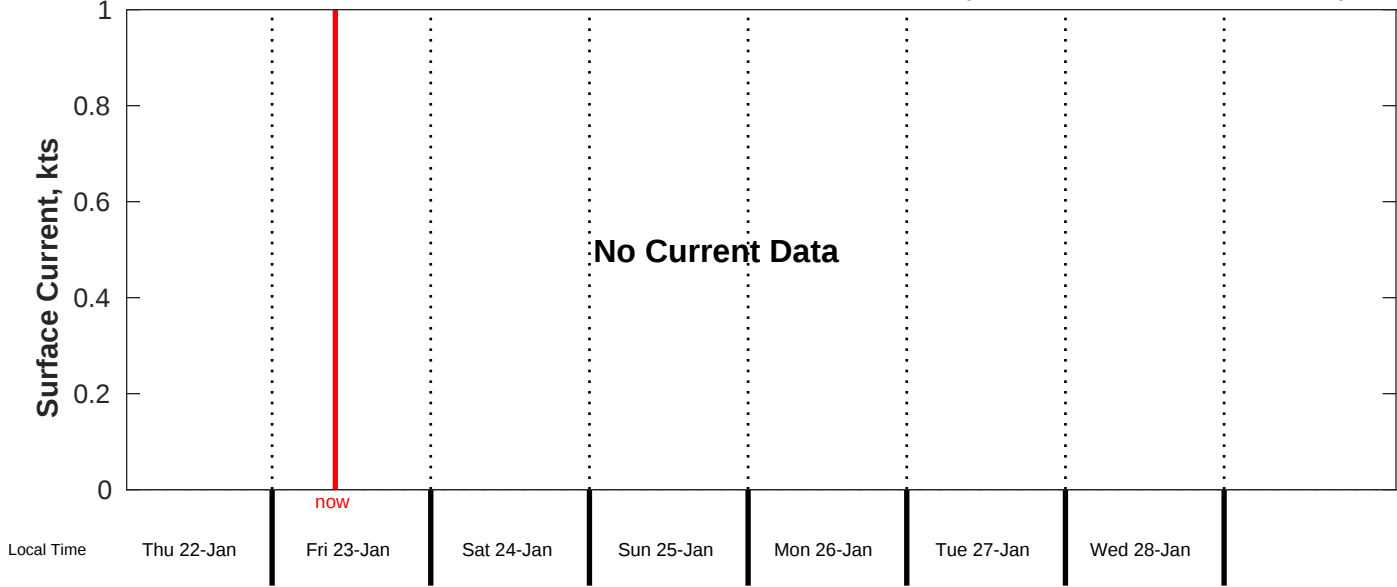
Surface Current Forecast for CSA (ONHYM) PPL EBS - Guinea from 22-Jan-2026 00:00:00 to 30-Jan-2026 00:00:00
