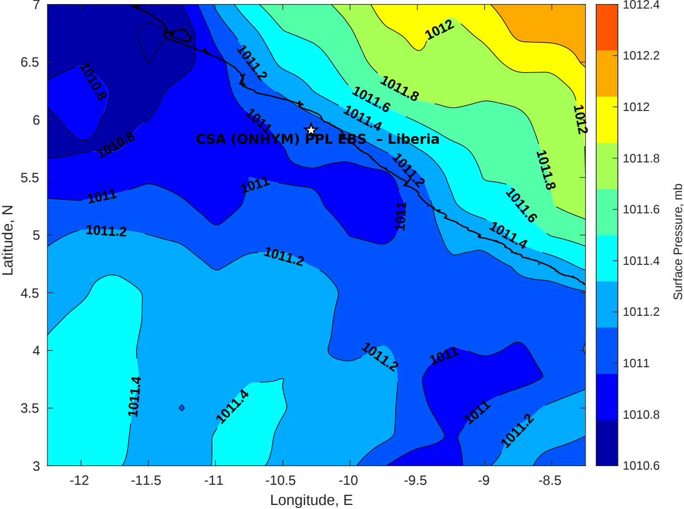
Surface Pressure (mb) for CSA (ONHYM) PPL EBS - Liberia at 23-Jan-2026 00:00:00
