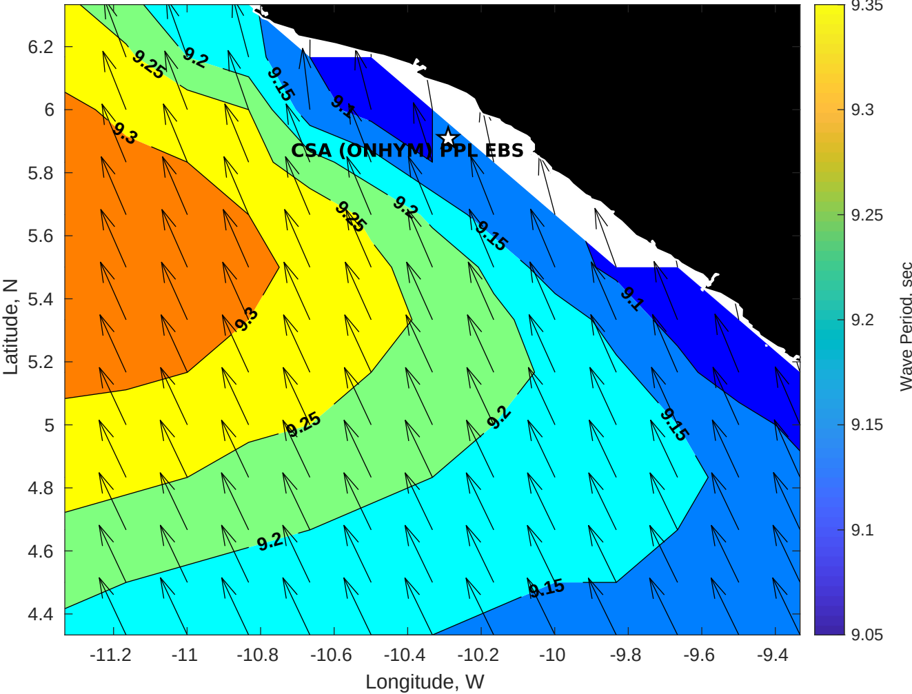
GFS Wave Period (sec) for CSA (ONHYM) PPL EBS - Liberia at 23-Jan-2026 09:00:00
