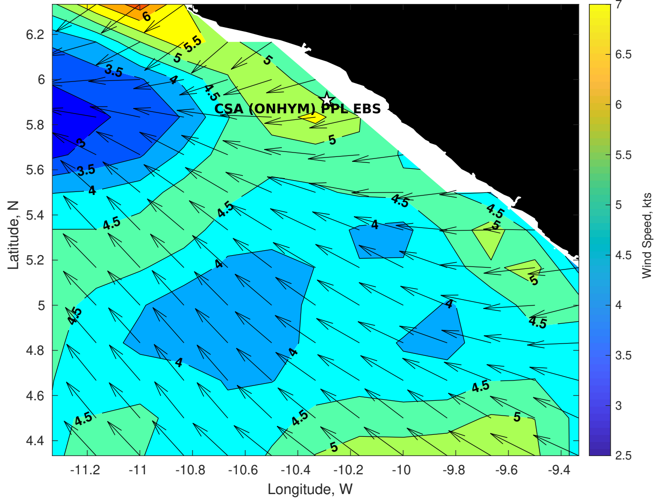
GFS Winds (kts) for CSA (ONHYM) PPL EBS - Liberia at 23-Jan-2026 09:00:00
