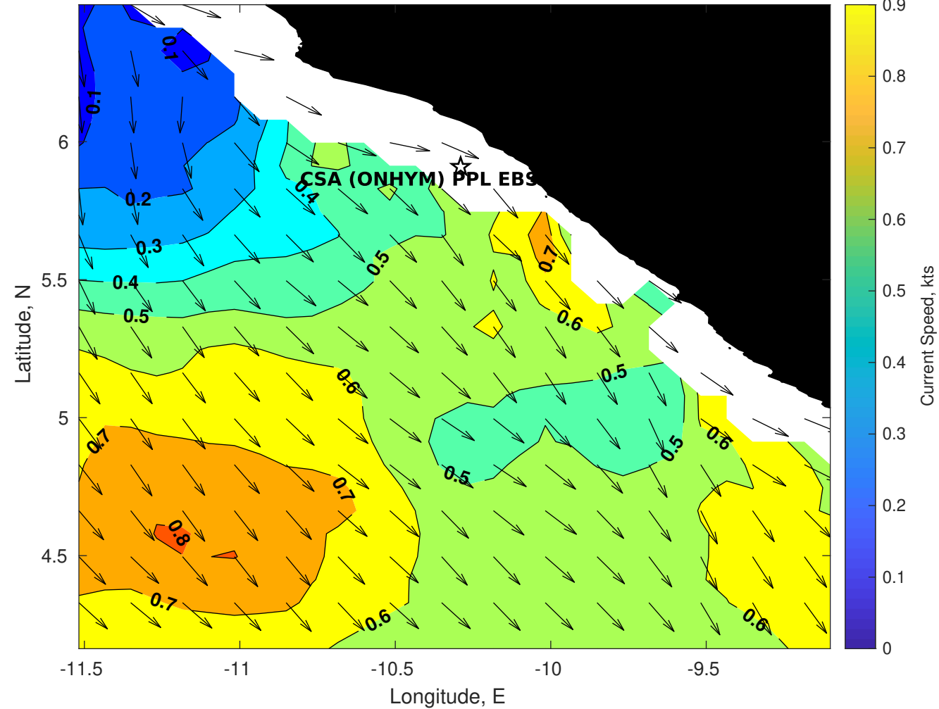
Surface Currents for CSA (ONHYM) PPL EBS - Liberia at 22-Jan-2026 00:00:00
