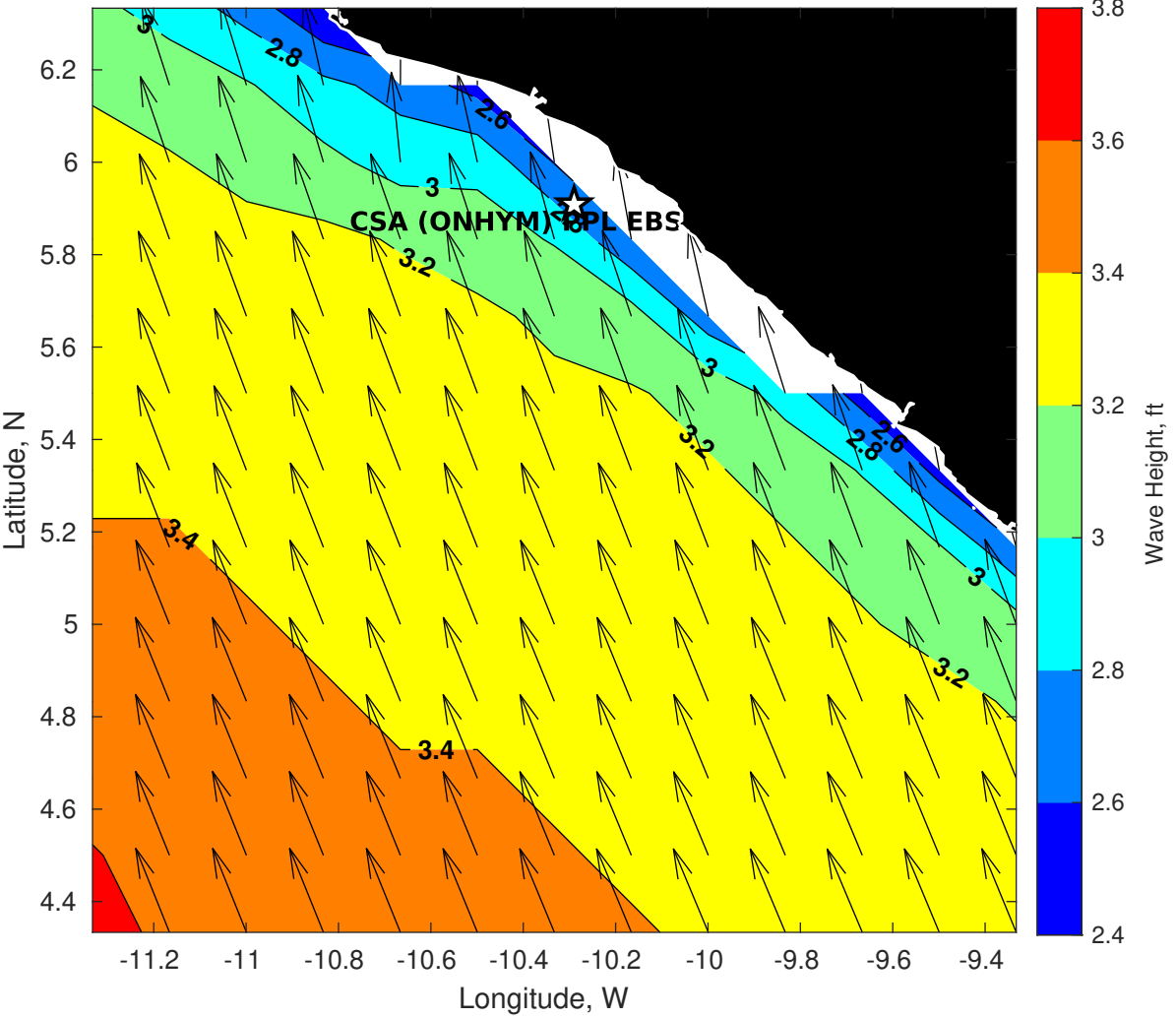
GFS Wave Height (ft) for CSA (ONHYM) PPL EBS - Liberia at 23-Jan-2026 09:00:00
