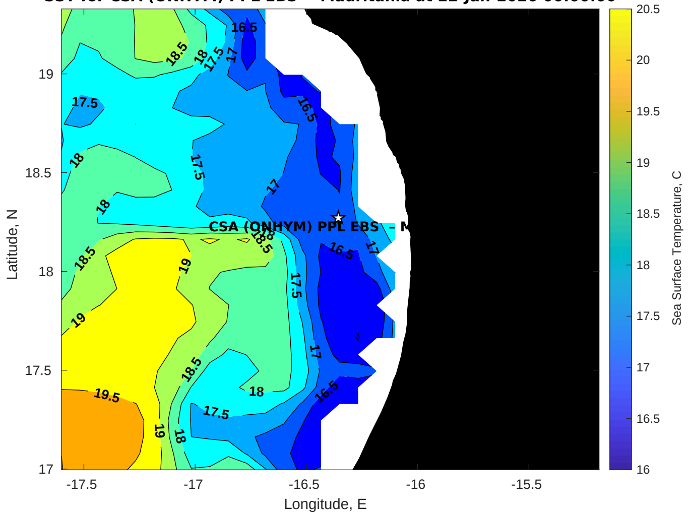
SST for CSA (ONHYM) PPL EBS - Mauritania at 22-Jan-2026 00:00:00
